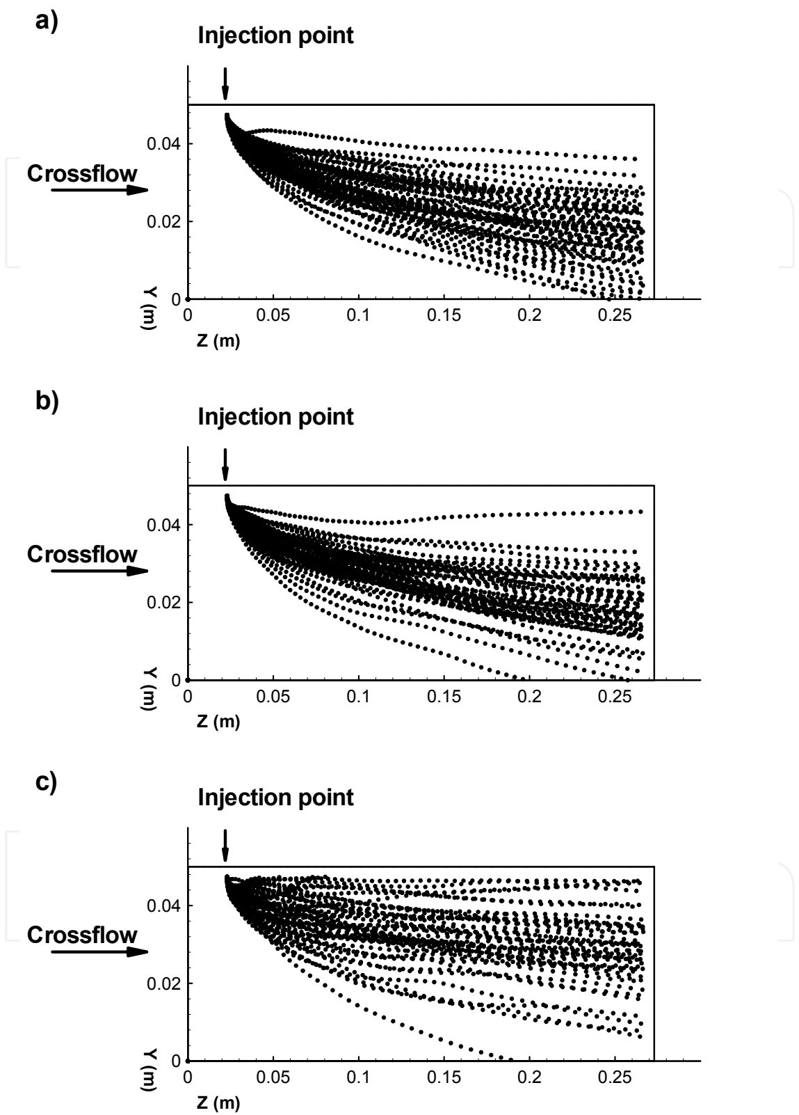
Fig. 5. Parallel projection of droplet trajectories in the vertical plane of symmetry ( X=0 ) for W_{cross}=10\text{m/s} and V_p=-1\text{m/s} and T_p=293K .: (a) Diesel fuel (DF-2), T_p=293K ; (b) RME, T_p=293K , (c) RME, T_p=443K .
