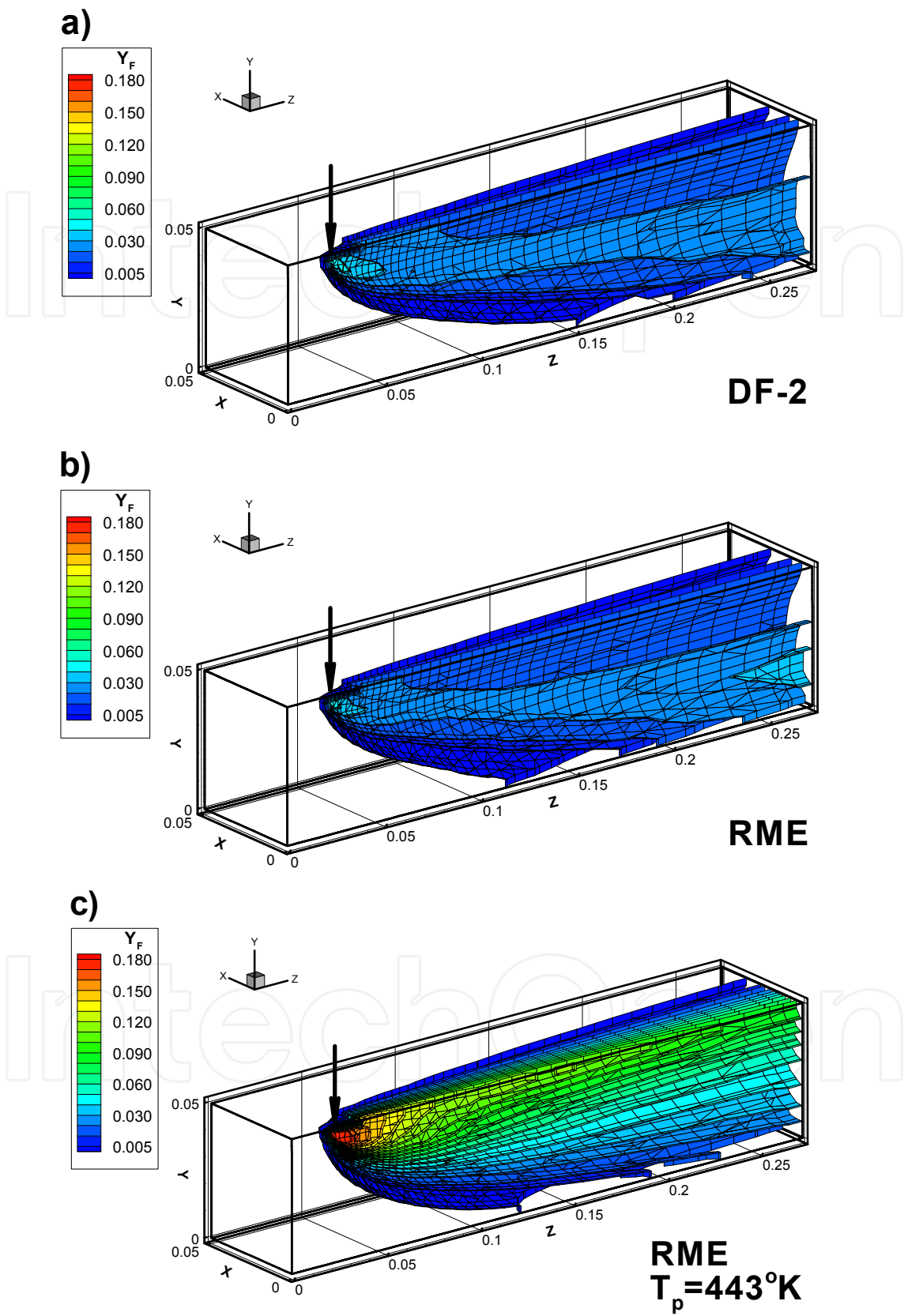
Fig. 6. Mass fraction distribution for W_{\text{cross}}=10\text{m/s} and V_p=-1\text{m/s} : (a) Diesel fuel (DF-2), T_p=293^\circ\text{K} ; (b) RME, T_p=293^\circ\text{K} , (c) RME, T_p=443^\circ\text{K} .
