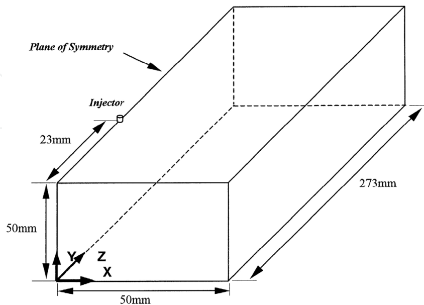
Fig. 1. Flow configuration
