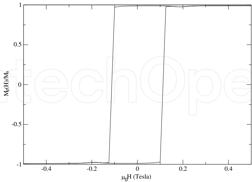
Fig. 2. Magnetic hysteresis loop of the z-component of the magnetic nanoparticle's magnetization in the case when the orientation of the magnetic anisotropy axis undergoes the small oscillations around the z-direction (parallel to the external dc magnetic field). Some parameters of the computer simulation: demagnetizing factor in shape anisotropy D = 0.15 ( K_a = \mu_0(1 - 3D)M_s^2/4 ), \alpha = 0.066 , R = 2\text{nm} , M_s = 450\text{kA/m} , T=10\text{K} .
