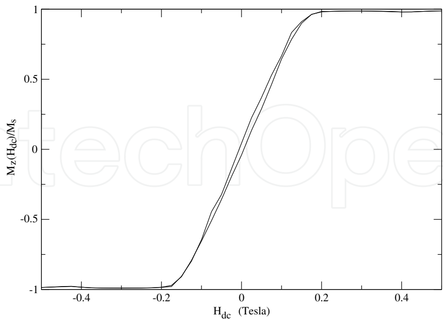
Fig. 3. The same as in Fig. 2 but the magnetic anisotropy axis orientation oscillates around the x-direction (transverse to the external dc magnetic field).
