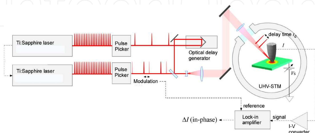
Fig. 9. Schematic illustration of SPPX-STIM
