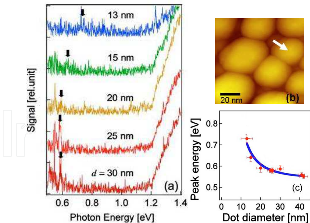
Fig. 3. (a) STM-PAS-FT spectra obtained from individual GeSn nanodots of various sizes. (b) Typical topographic STM image of Ge 1-x Sn x nanodots. The white arrow indicates the position where the spectrum for d=30 nm was acquired. (c) Peak energy in (a) as a function of the lateral diameter of the nanodots. The solid curve is calculated from Eq. (1). [10]
