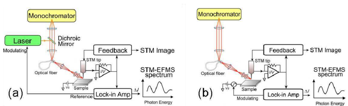
Fig. 4. Schematic illustrations of STM-EFMS measurement: (a) OM scheme, (b) BM scheme.[15]*
