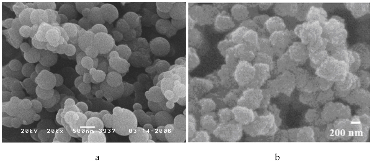
Fig. 2. Scanning electron micrograph of calcined mesoporous silicas a) NanocrystallineMCM-41 and b) Nanohollow cuboids
