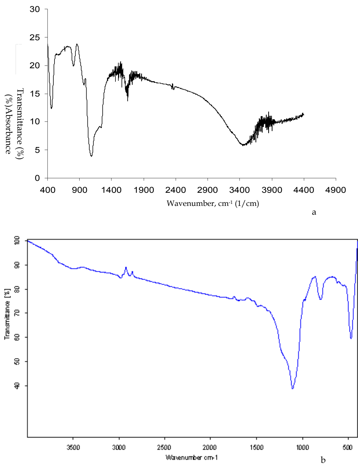
Fig. 6. Fourier transform Infrared spectroscopic analysis of as-synthesized mesoporous silicas, a) Nanohollow cuboids and b) a) Nanocrystalline MCM-41.
