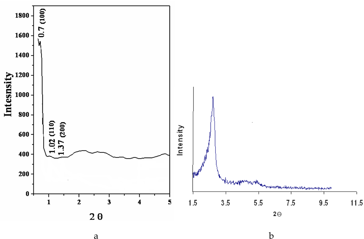
Fig. 1. X-ray diffraction pattern of calcined mesoporous silicas a) Nanohollow cuboids and b) Nanocrystalline MCM-41
