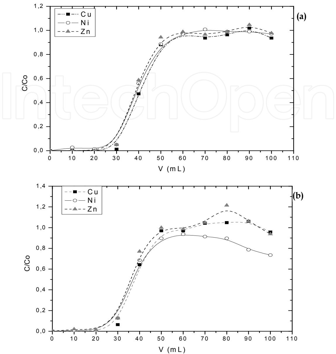
Fig. 11. Breakthrough curves of metals. (a) wastewater with cyanide (18 mg/L) and (b) wastewater after NaOCl oxidation of cyanide. Amount of adsorbent 4.0g, \text{Cu}^{+2} concentration 200 mg/L at pH 1.78 and flow rate of 2.0mL/min. C/C_0 represent the ion concentrations for initial and final solution. (Adaptaded from Sousa et al., 2009. Journal Environment Manager, Vol. 90, N° 11, pp. 3340–3344, ISSN 0301-4797)
