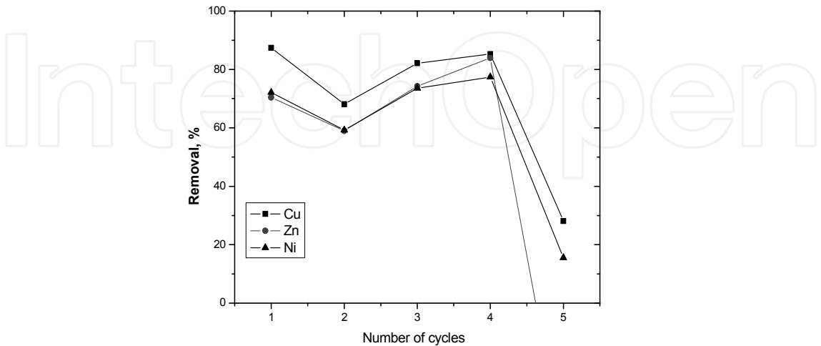
Fig. 12. Removal efficiency with number of cycles for metal ions on cane sugar bagasse from wastewater ((Adaptaded from Sousa et al., 2009. Journal Environment Manager, Vol. 90, N° 11, pp. 3340-3344, ISSN 0301-4797)
