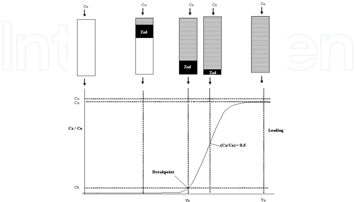
Fig. 10. Ideal breakthrough curve. (Adaptaded from Cooney, D.O.(1999). Adsorption design for wastewater treatment , Lewis publishers, ISBN 1566703336 9781566703338. Boca Raton, Fl and McKay, G. (1996) (Editors), Design of adsorption contatacting systems,in: Use of Adsorbents for the Rremoval of Pollutans from Wasterwaters ,pp 99-131,CRC press,Inc, Boca Raton, Florida ISBN: 0-8493-6920-7
