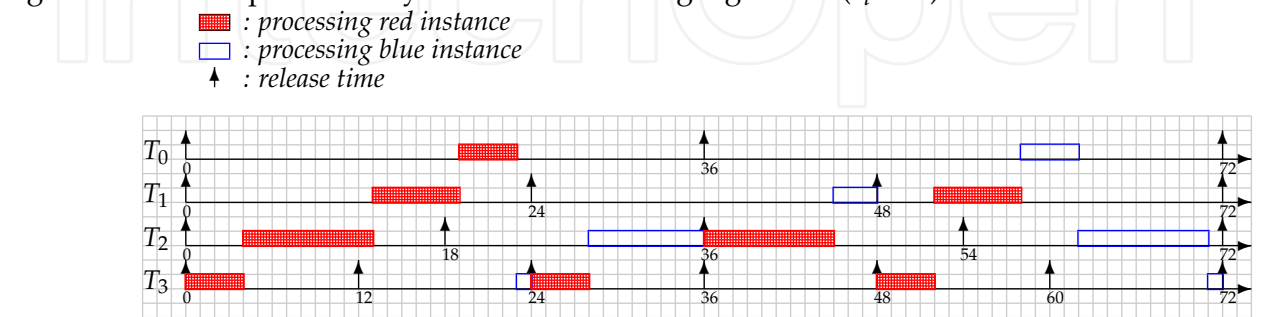
Fig. 4. A schedule produced by the BWP scheduling algorithm ( s_i = 2 )
