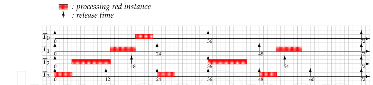
Fig. 3. A schedule produced by the RTO scheduling algorithm ( s_i = 2 )
