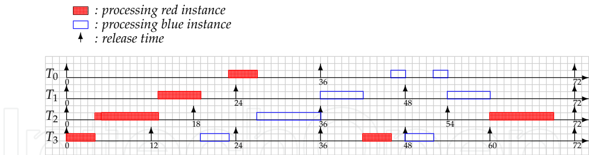
Fig. 8. A schedule produced by the RLP/T scheduling algorithm ( s_i = 2 )
