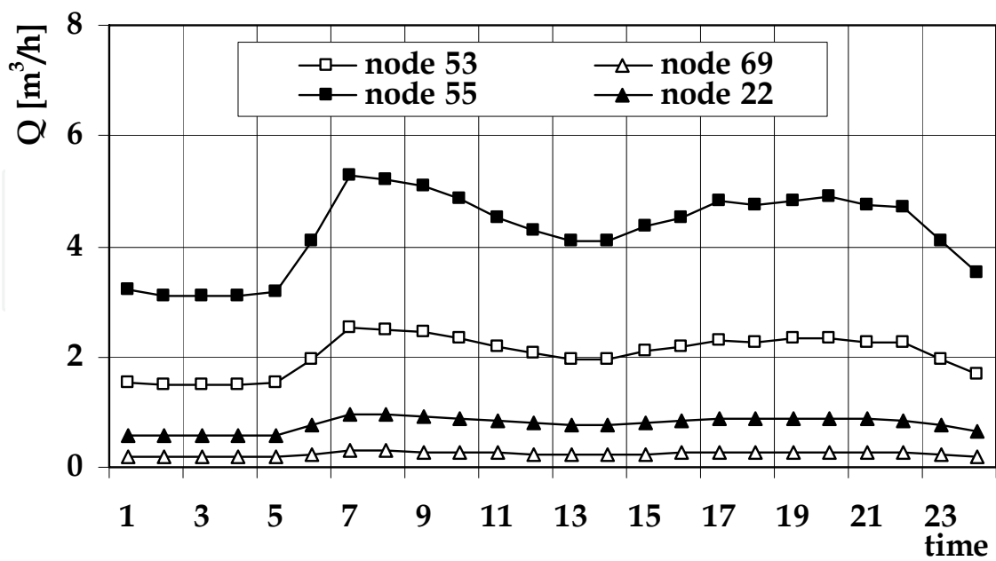
Fig. 7. Change of the gas stream size Q leaving the network in four exemplar nodes of the network in particular hours of the day; air temperature t = -4\text{ }^{\circ}\text{C} .
