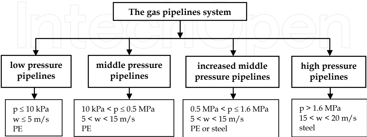
Fig. 2. The main types of gas pipeline networks.
