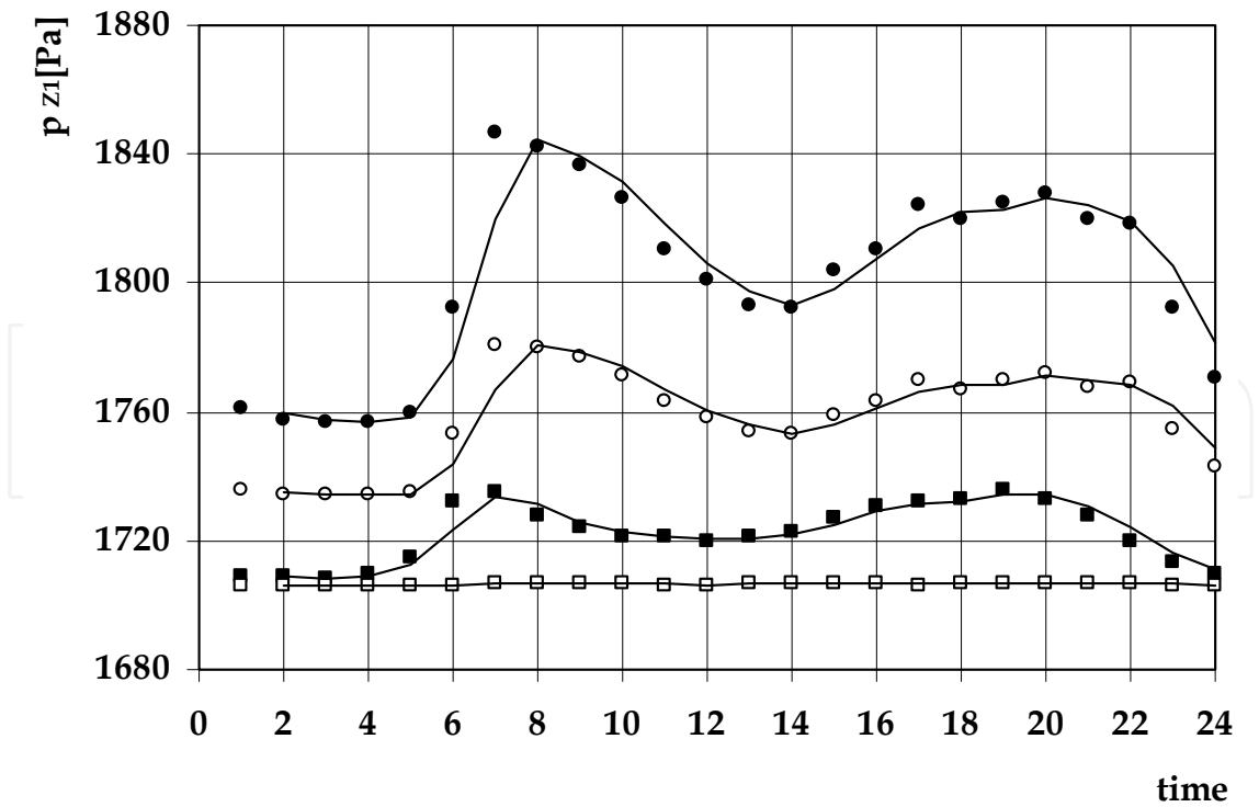
Fig. 10. The change of the gas stream overpressure p_{z1} feeding the network in particular hours of the day; various values of air temperature; (●) t = -16^\circ\text{C} , (○) t = -4^\circ\text{C} , (■) t = 8^\circ\text{C} , (□) t \geq 18^\circ\text{C} .
