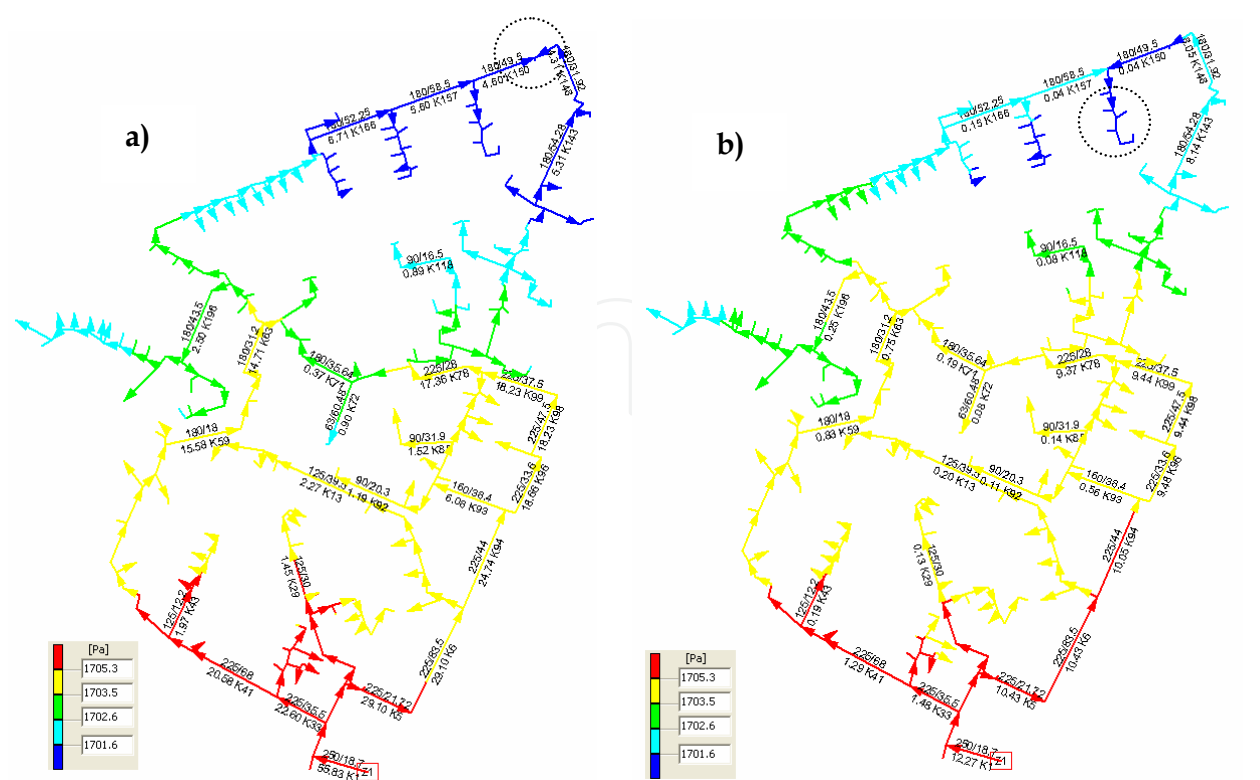
Fig. 13. Gas stream overpressure arrangement in pipelines network; t \geq 18 °C; a) results for 7 am ( p_{z1} = 1707 Pa; Q_{feed} = 55.83 m³/h); b) results for 3 am ( p_{z1} = 1706 Pa; Q_{feed} = 12.27 m³/h).
