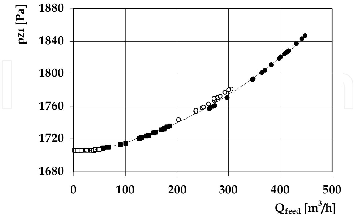
Fig. 9. The effect of gas stream size feeding the network Q_{feed} on the gas stream overpressure p_{z1} ; (●) t = -16^\circ\text{C} , (○) t = -4^\circ\text{C} , (■) t = 8^\circ\text{C} , (□) t \geq 18^\circ\text{C} .
