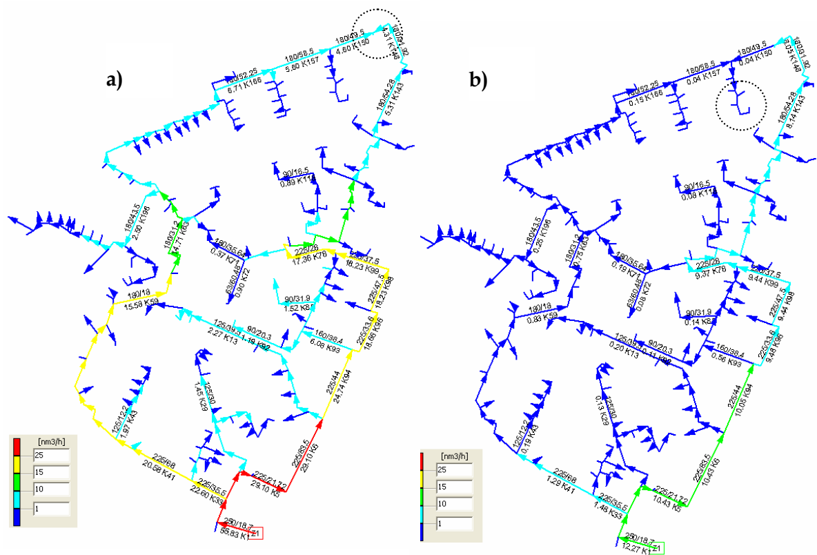
Fig. 11. Gas stream arrangement in pipelines network; t \geq 18 °C; a) results for 7 am ( p_{z1} = 1707 Pa; Q_{feed} = 55.83 m³/h); b) results for 3 am ( p_{z1} = 1706 Pa; Q_{feed} = 12.27 m³/h).
