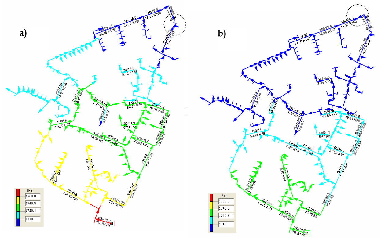
Fig. 14. Gas stream overpressure arrangement in pipelines network; t = -4 °C; a) results for 7 am ( p_{z1} = 1781 Pa; Q_{feed} = 312.07 m³/h); b) results for 3 am ( p_{z1} = 1734 Pa; Q_{feed} = 186.80 m³/h).
