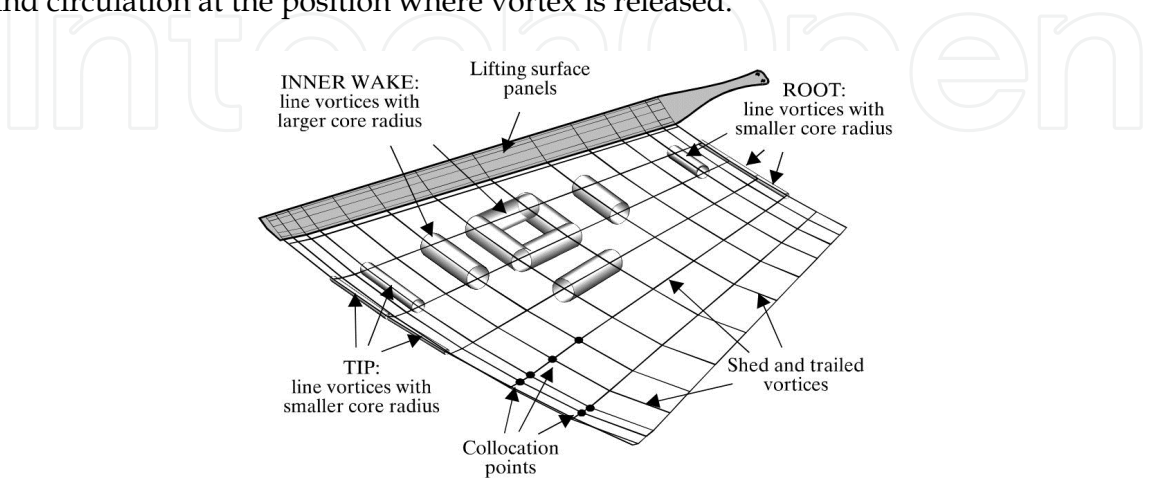
Fig. 17. Discretized wake
