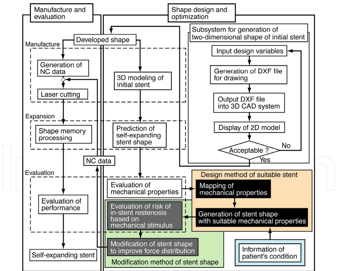
Fig. 8. Design support system for self-expanding stent. The left-hand side shows the production process of the SENDAI stent. The right-hand side shows the flow of the proposed design support system.
