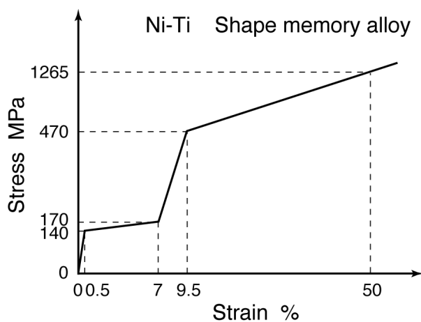
Fig. 10. Assumed stress-strain relationship for the stent material
