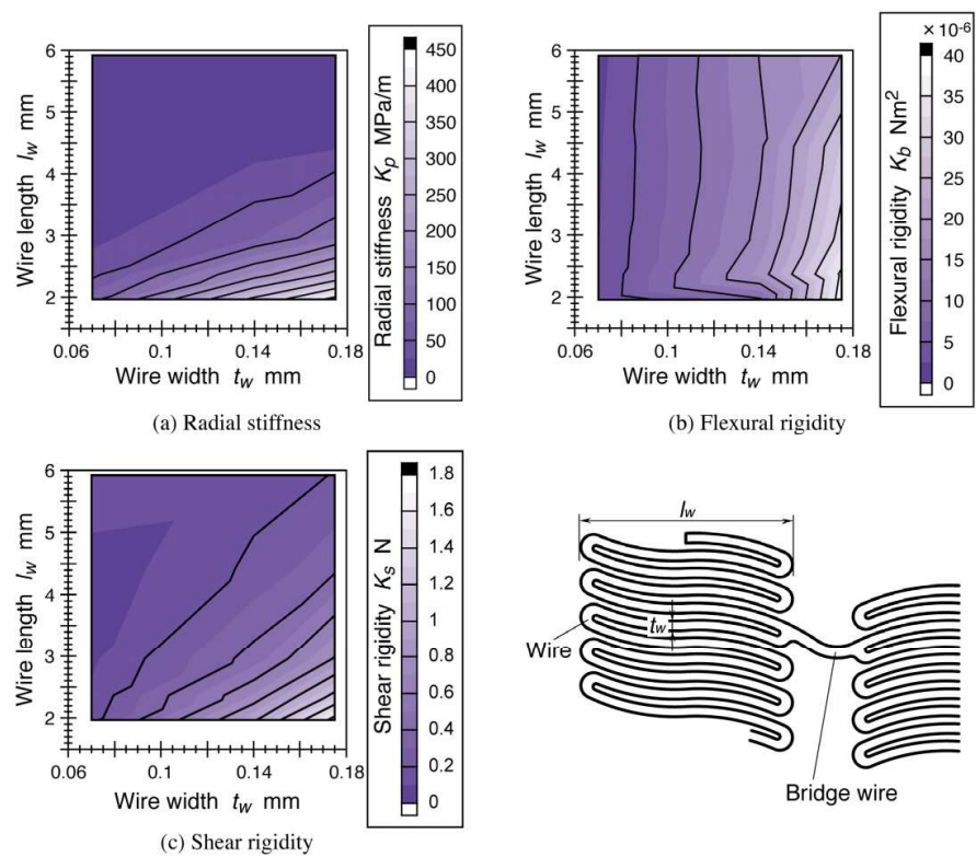
Fig. 9. Sensitivities of the mechanical properties of the SENDAI stent 6 mm diameter to the design variables: (a) radial stiffness, (b) flexural rigidity, and (c) shear rigidity
