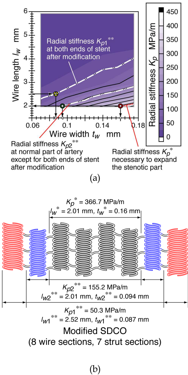
Fig. 20. The SDCO stent 6 mm in diameter is modified to suit the assumed symptom of the coronary artery. (a) Design variables after modification are determined by using the map of the radial stiffness. (b) The modified SDCO has a nonuniform shape along its axial direction.
