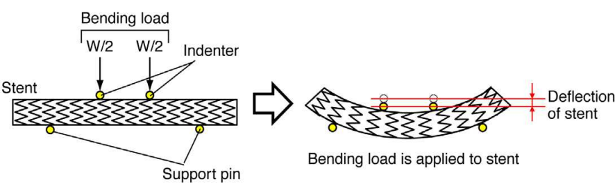
Fig. 3. Schematic view of the bending test
