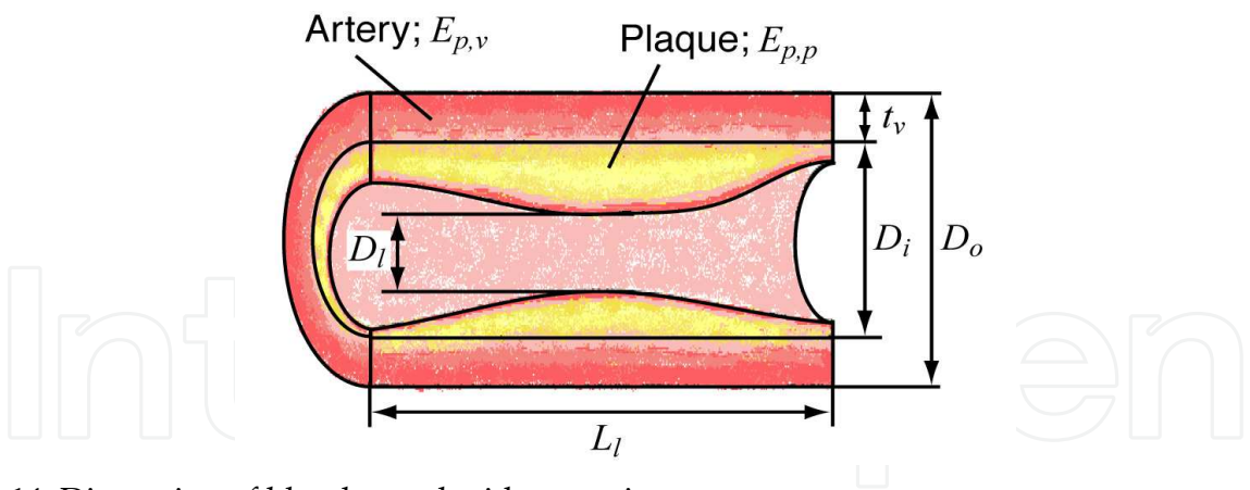
Fig. 14. Dimension of blood vessel with stenosis
