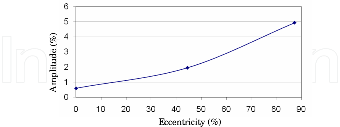
Fig. 17. Failure amplitude vs. eccentricity There is a clear relationship between the failure amplitude and the amount of eccentricity (Table 8) (Fig. 17). In Fig. 18 the induced eccentricity failure. The methodology proposed in this work is capable of detecting eccentricity failures and its evolution as a function of the defect amplitude. It should be noted however, that the tests
