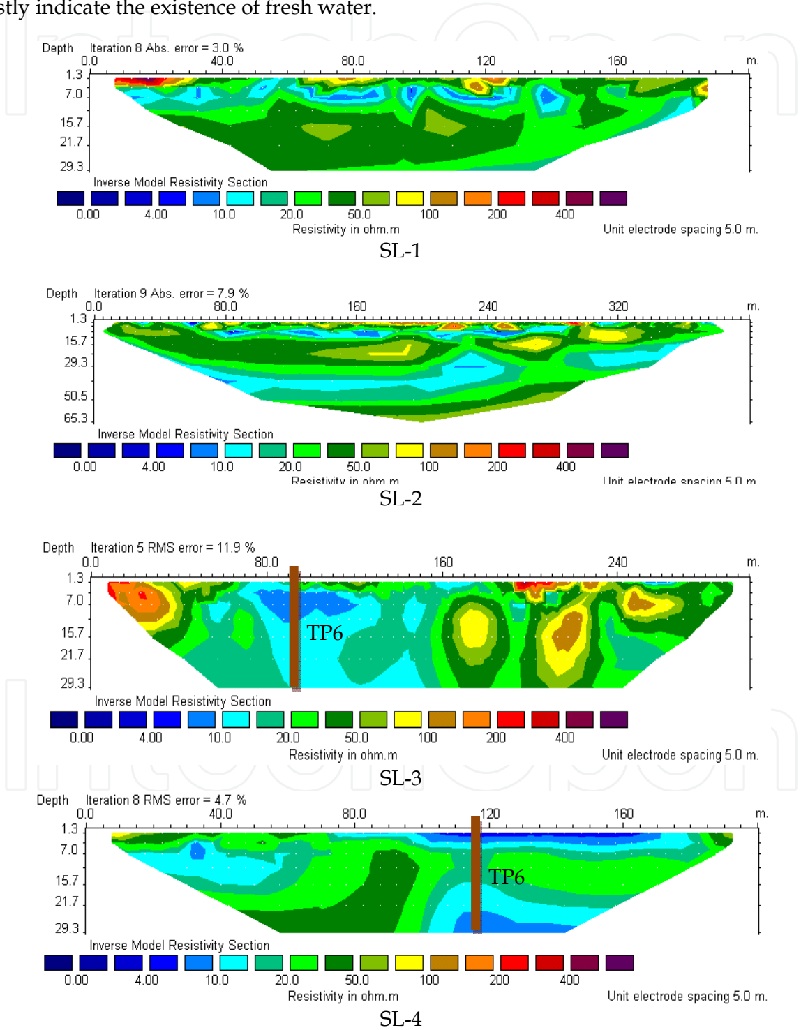
Fig. 6. Profile of ERI survey lines at the sorrounding of waste disposal area
