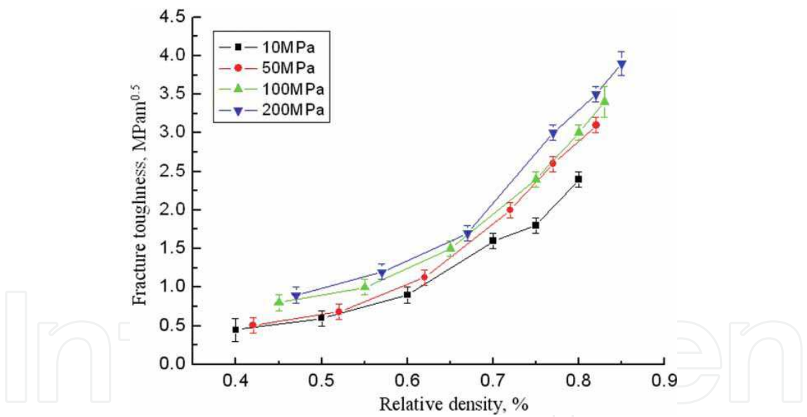
Fig. 7. Dependence of fracture toughness on relative density of TiB2 porous ceramic
