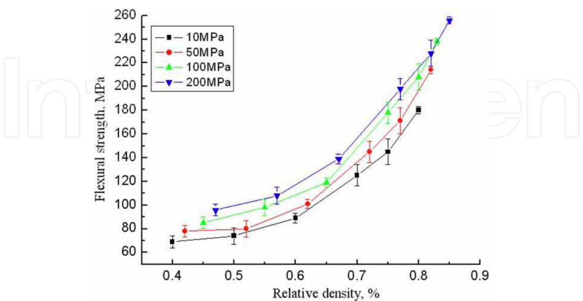
Fig. 6. Dependence of flexural strength on relative density of TiB2 porous ceramic
