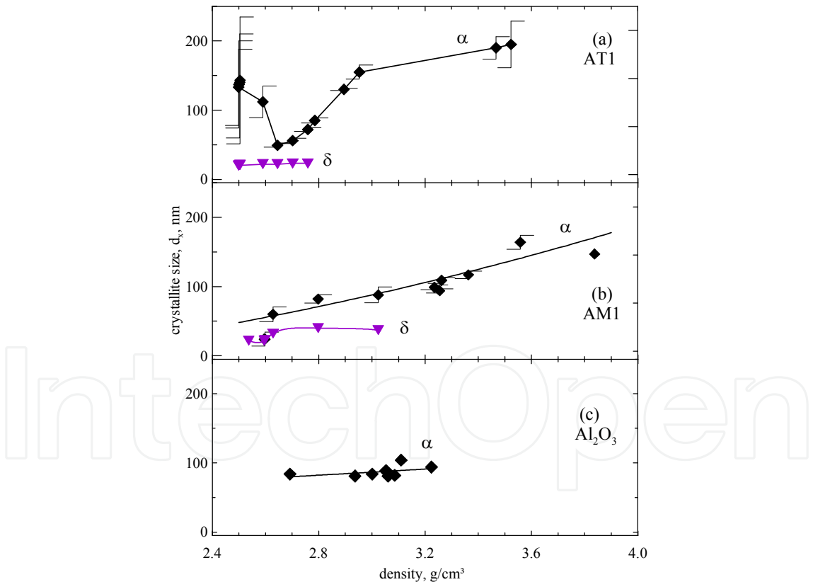
Fig. 8. Average X-ray crystallite size evolution upon sintering of the alumina ceramics, doped with: (a) - titania, AT1, (b) - magnesia, AM1, (c) - \text{Al}_2\text{O}_3 without dopants; constant heating rate 10^\circ\text{C}/\text{min} .
