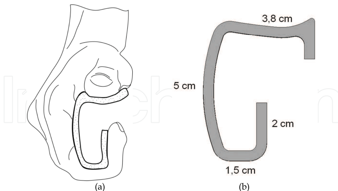
Fig. 10. Applying ergonomics: (a) preliminary proposal for the pushrim design; (b) defined project: shape and dimensions (Medola et al., 2011).
