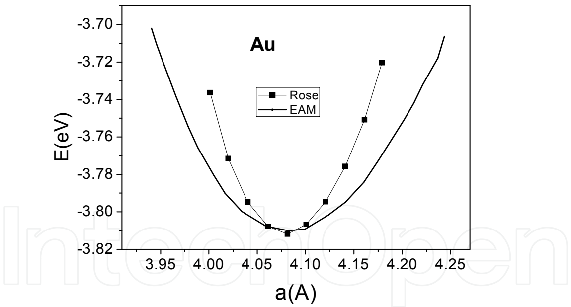
Fig. 1. Rose and EAM energies versus lattice constant for Au.
