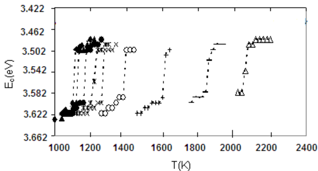
Fig. 4. The cohesive energy as a function of temperature at different pressure for Au. The symbols \blacklozenge, \blacktriangle, \bullet, \times, \times, \circ, + represents the pressure values of 0.0, 0.5, 1.0, 1.5, 2.5, 5.0, 7.5 GPa, respectively.
