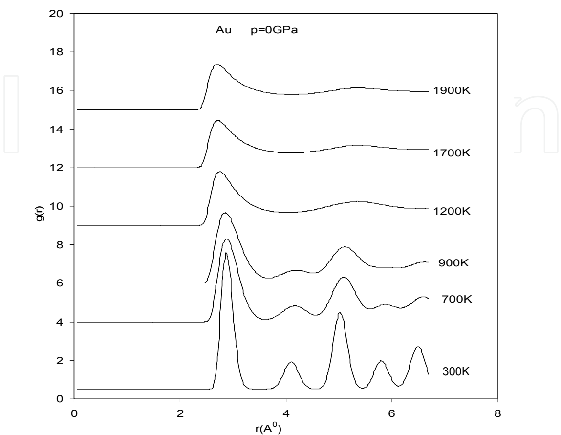
Fig. 5. The radial distribution curves in solid and liquid phases for Au.
