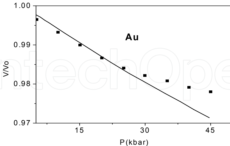
Fig. 7. Variation of pressure as a function of V/V_o for Au. Experimental points are taken from Ref.[37].
