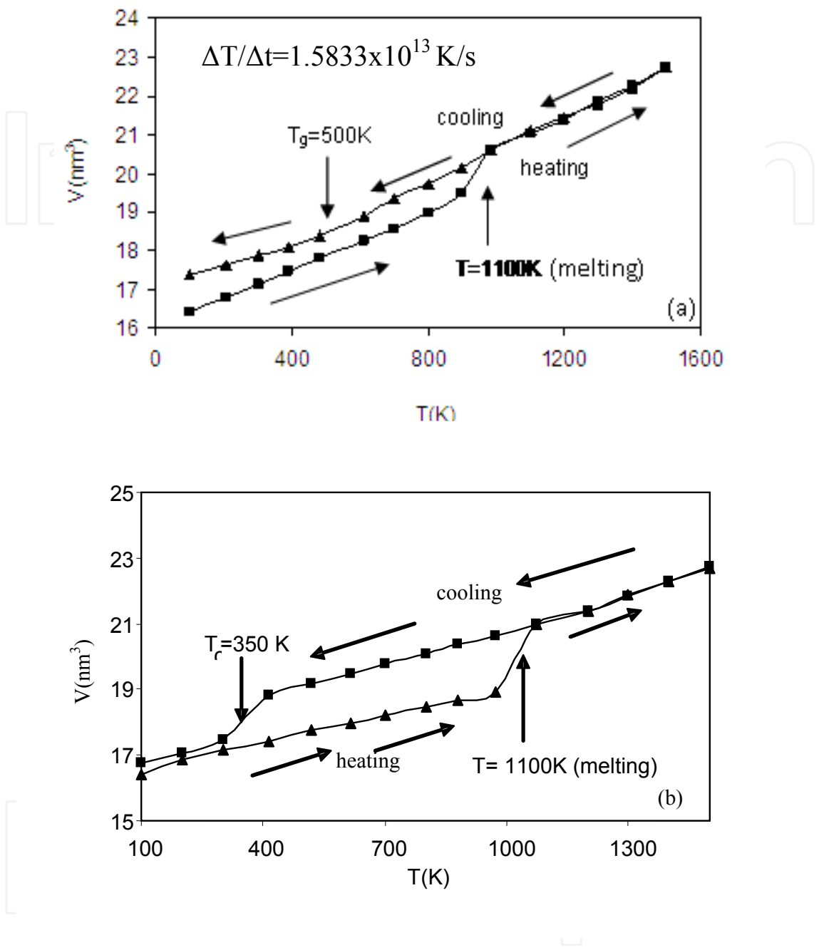
Fig. 8. Average volume of Au during heating and cooling at a rate of (a) 1.5833 \times 10^{13} \text{ K/s} and (b) 1.5833 \times 10^{12} \text{ K/s} .
