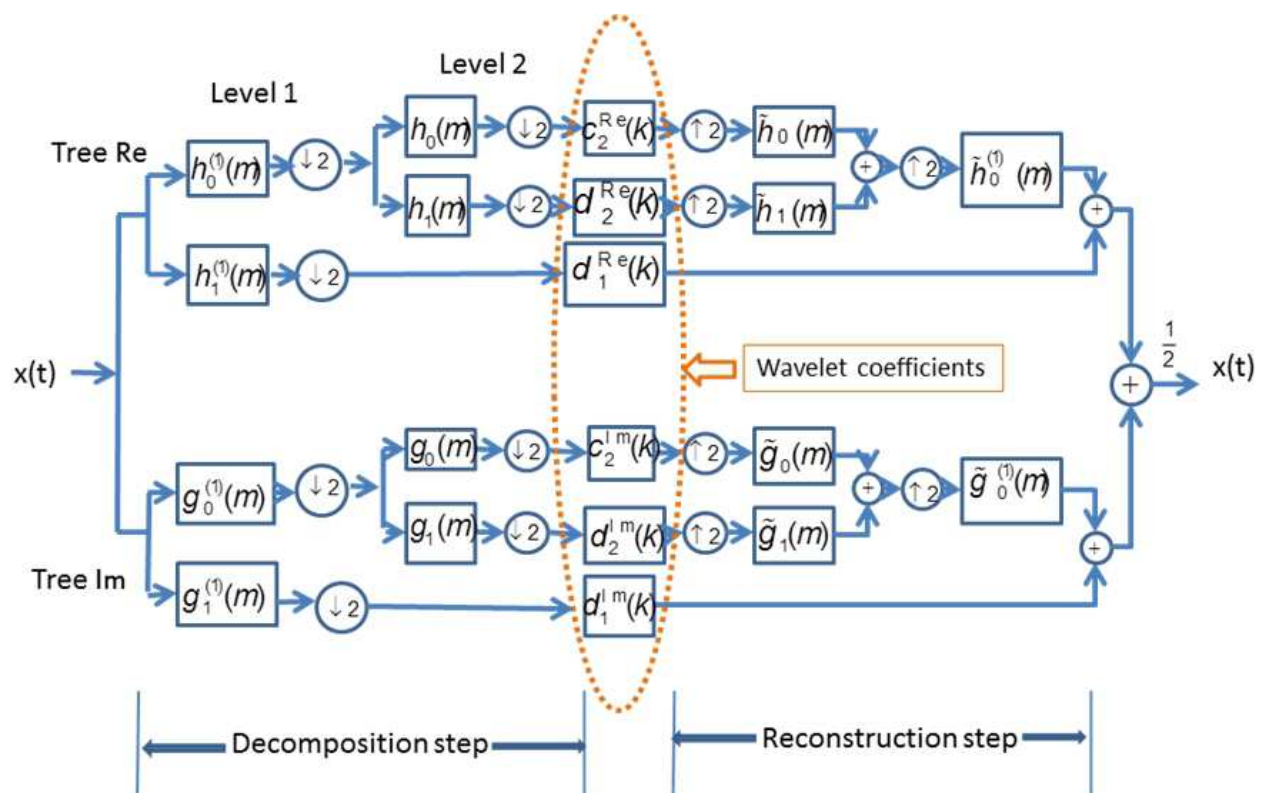
Fig. 3. Decomposition and reconstruction stages of DTCWT
