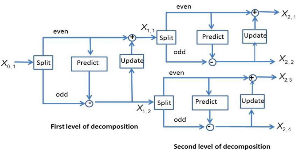
Fig. 7. Decomposition step of SGWPT
