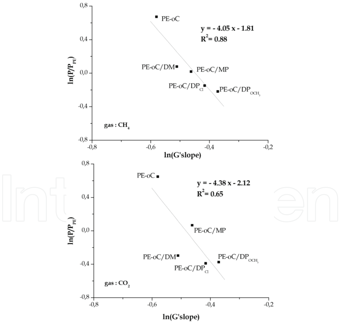
Fig. 13. Comparison of CH 4 and CO 2 permeabilities with G' slopes.
