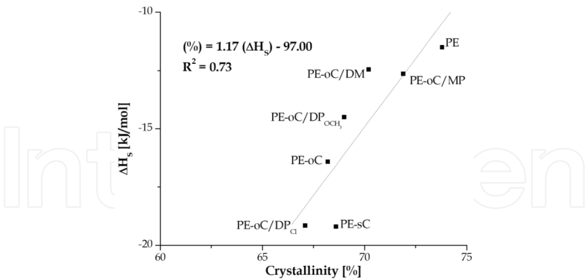
Fig. 12. Degree of crystallinty vs. Enthalpy of Solubility.
