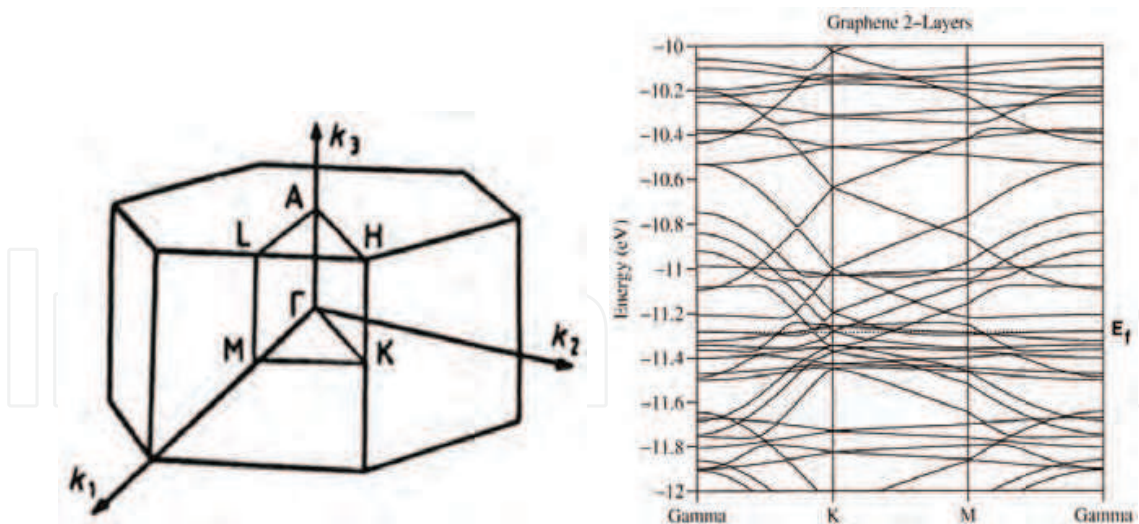
Fig. 4. Energy bands for graphene 2-L. The inset depicts the Wigner-Seitz cell for a hexagonal configuration.
