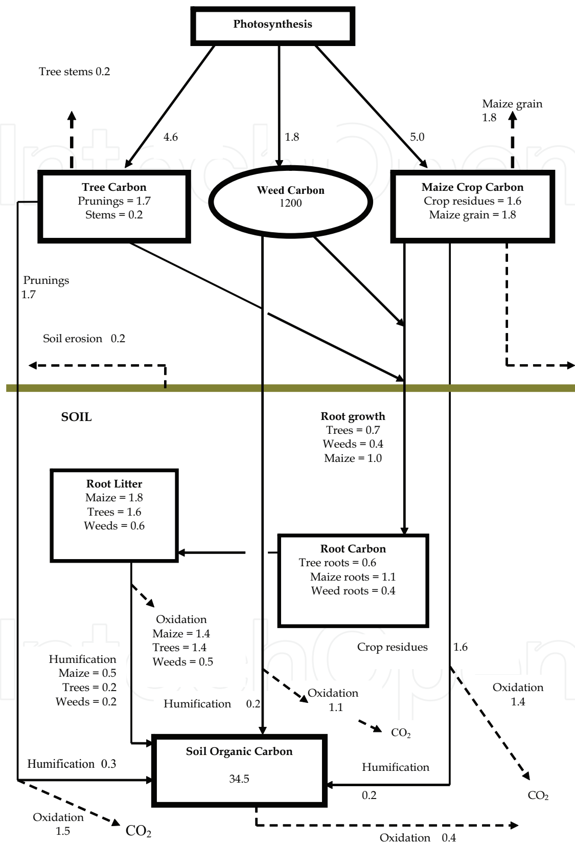
Fig. 4. A conceptual model of the carbon cycle in the tree-maize intercropping phase of a coppicing improved fallow. Values are in \text{kg C ha}^{-1} and \text{kg ha}^{-1} \text{ yr}^{-1}
