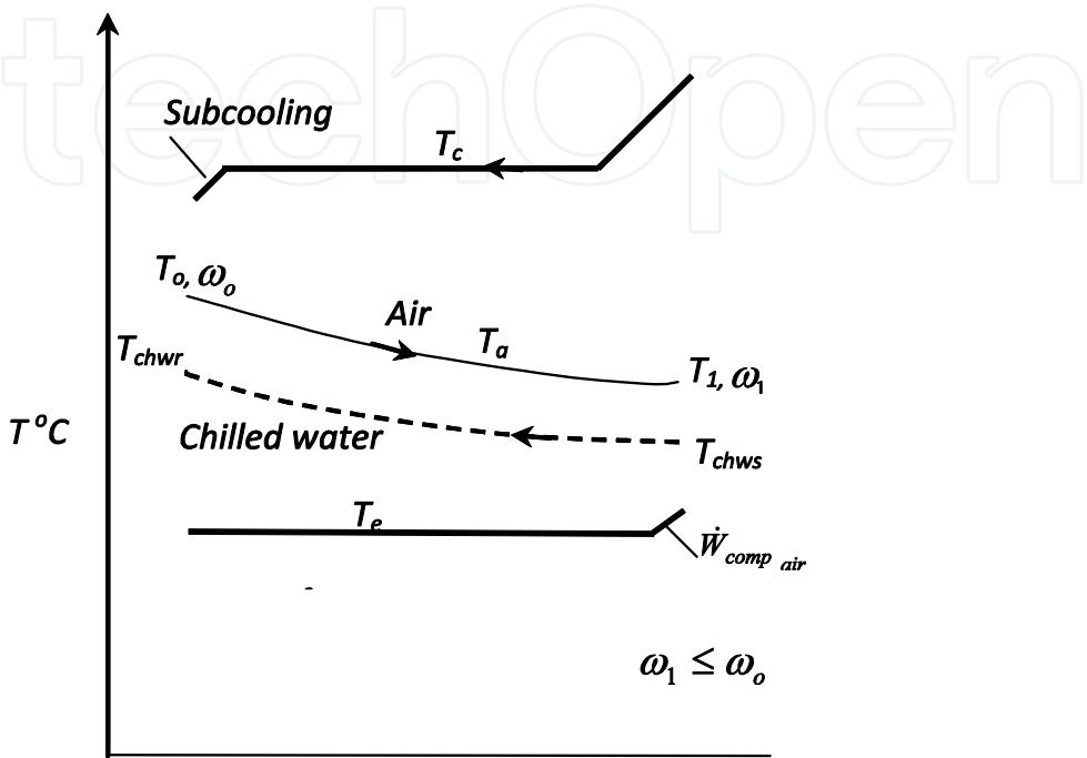
Fig. 2. Temperature levels for the three working fluids, not to scale
