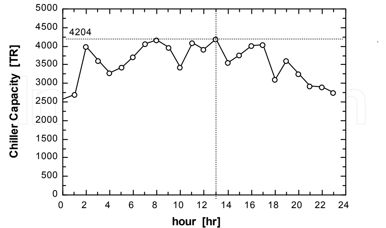
Fig. 6. Chiller capacity variation with the climatic conditions of the selected design day
