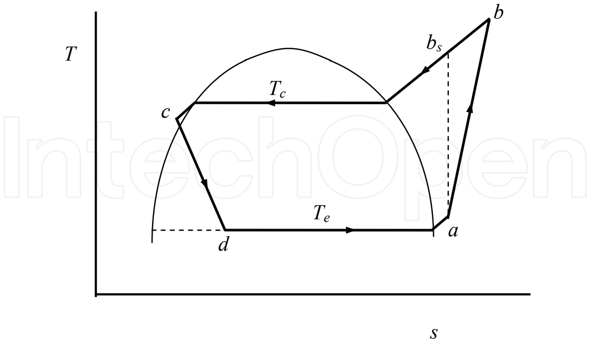
Fig. 1c. T - s diagram for a refrigeration machine
