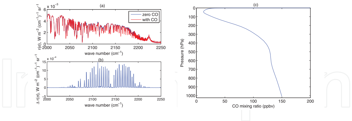
Fig. 9. The figure shows (a) two synthetic IASI spectra in the spectral region of CO absorption; one of the spectra has been calculated with zero load of CO. (b) The difference between the two evidences the sinusoidal appearance of the CO absorption features. Panel (c) shows the CO reference profile used for radiative transfer calculations.
