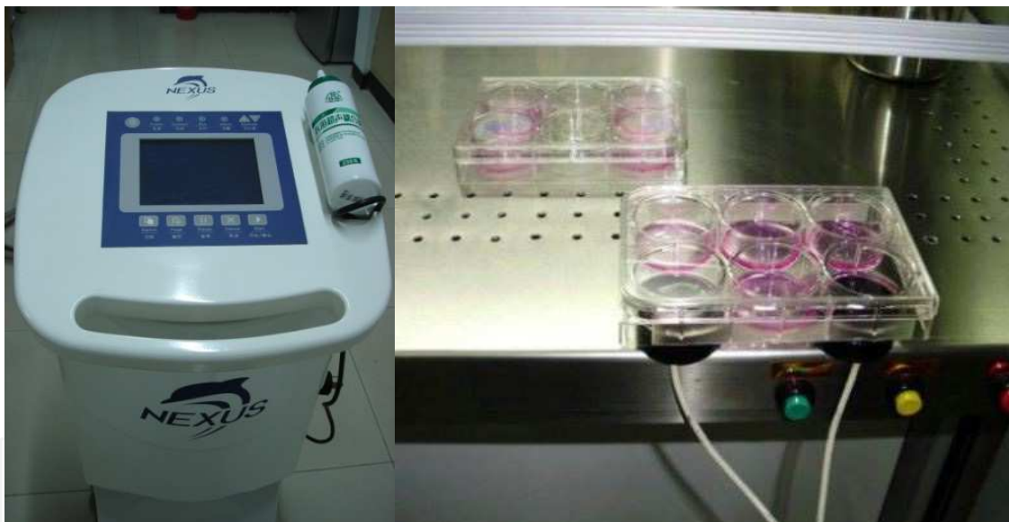
Fig. 1. Experimental apparatus for applying low- intensity pulsed ultrasound (LIPUS) which generated LIPUS with a SATA intensity of 10 \text{ mW/cm}^2 , pulse width of 200 microseconds, repetition rate of 1.5 KHz, and an operation frequency of 1MHz. LIPUS irradiated neurons with two probes 24 h after in culture. A six-well plate was placed on the probes. LIPUS was transmitted to culture plate via an interposed ultrasound gel. Two transducers for the control group (sham-LIPUS; LIPUS not turned on) and two probes for the LIPUS group.
