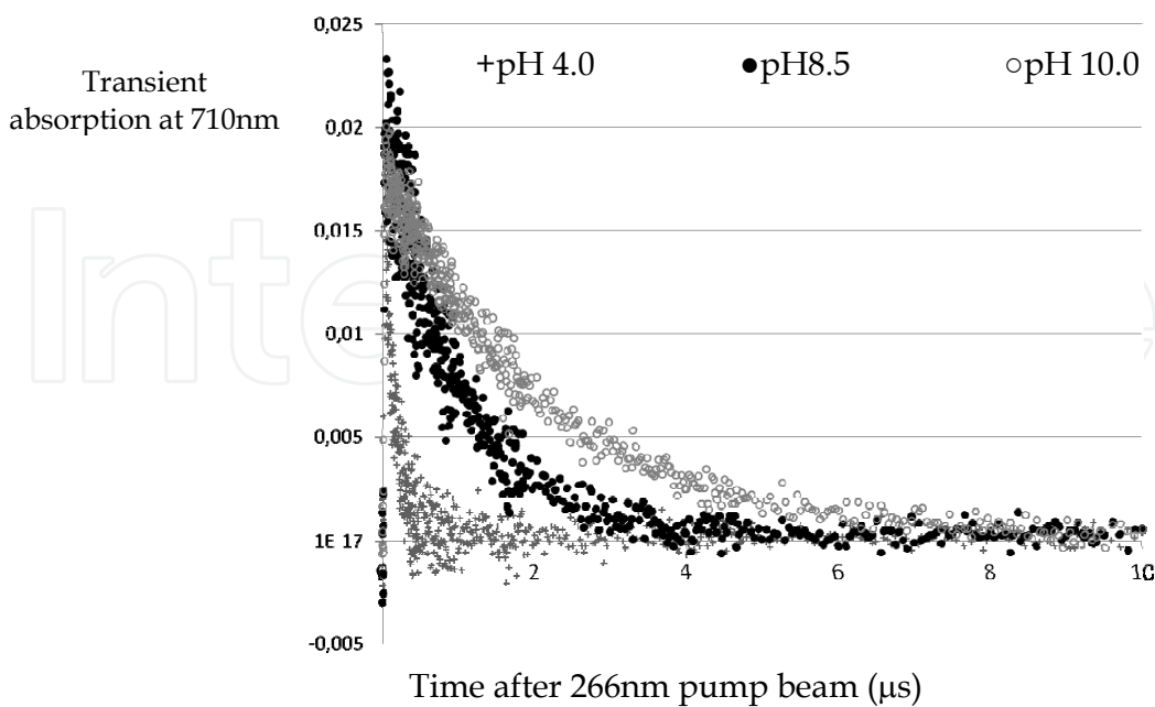
Fig. 4. Decay kinetics of the solvated electron absorption peak at 710nm within 10μs after excitation.
