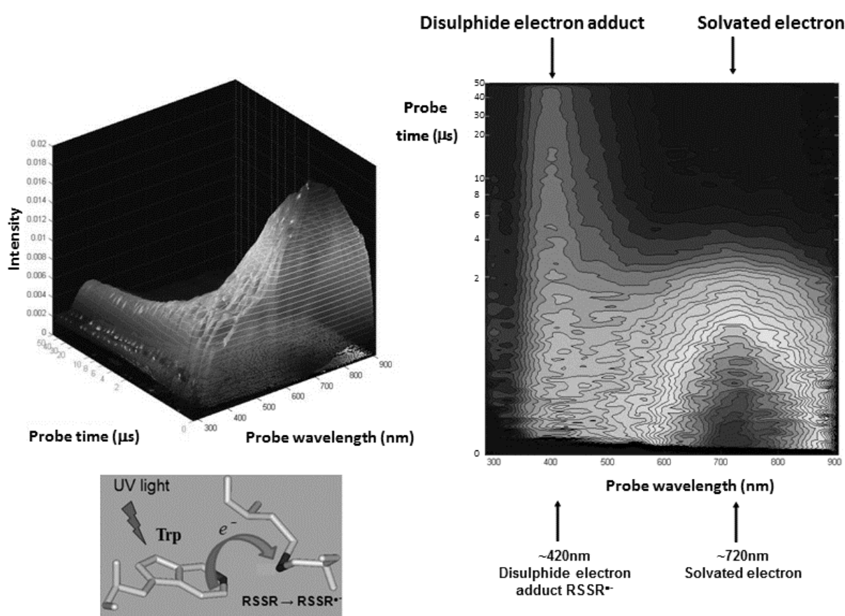
Fig. 2. Cutinase transient absorption data. Transient absorption data collected at probe times from 0 to 50 \mu\text{s} . The transient solvated electron absorbs maximally light at ~710-720nm (intense peak) and the disulphide bridge electron adduct radical has its maximum absorption at ~420nm. The intensity of the peaks displayed in the 2D image to the right can be seen in the 3D image to the left.
