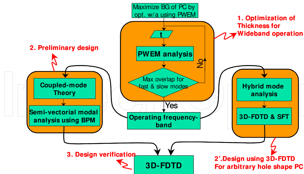
Fig. 4. The flow chart of the design methodology of PC slab waveguide based polarization rotator.
