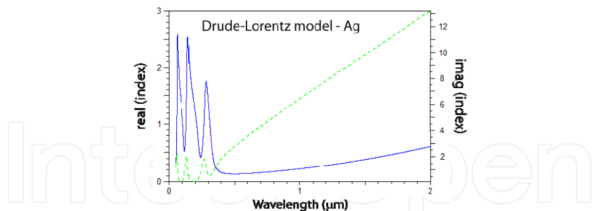
Fig. 2.10. Real (continuous/blue line) and imaginary (dashed/green line) parts of Ag refractive index for the Drude-Lorentz model. Three resonant peaks are shown in the UV region. Silver plasma frequency \omega_p=9.04\text{eV}\sim137\text{nm} .
