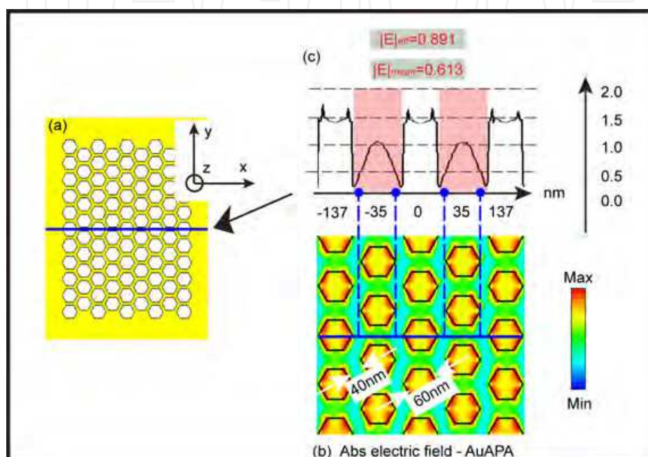
Fig. 3.3. a) The overall honeycomb structure. b) The overall electric field distribution in x-y plane, in this case, the polarization of incident light is along x-direction; c) absolute value of the electric field profile along the highlighted horizontal line. The excitation light is \lambda = 633 nm on gold surface with dielectric function \epsilon_{real} = 9.83 and \epsilon_{imaginary} = 1.97 .
