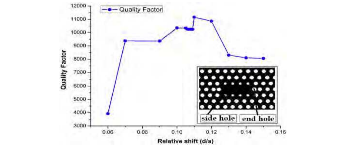
Fig. 11. Quality factor as function of the shift of the nearest holes of the L3 cavity. Inset:schematic diagram of the L3 cavity modified with different value for the holes in the first lines next to the cavity
