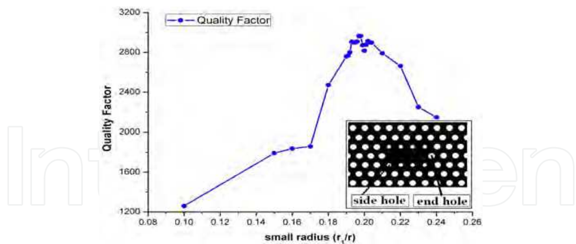
Fig. 10. Quality factor as function of the radius of the nearest holes of the L3 cavity. Inset:schematic diagram of the L3 cavity modified with different value for the holes in the first lines next to the cavity
