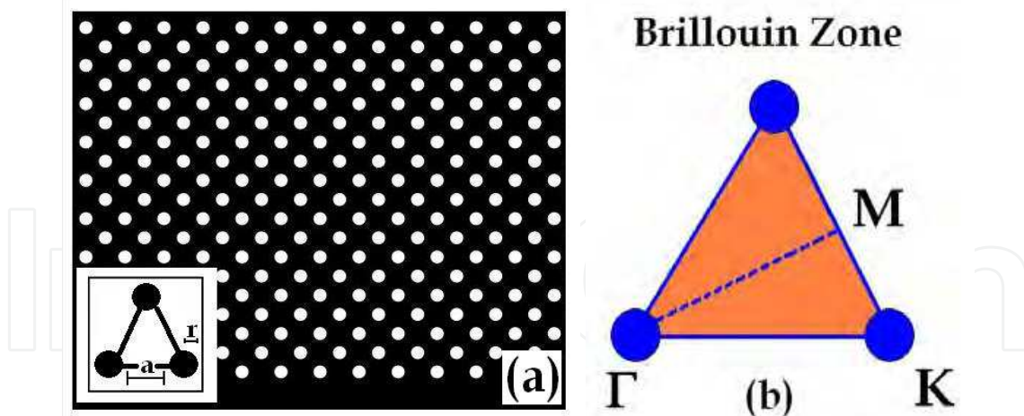
Fig. 6. a) two dimensional hexagonal array: (inset Primitive cell of the two dimensional hexagonal array showing lattice spacing a and radius r ). b) First Brillouin Zone showing the critical points \Gamma , K and M
