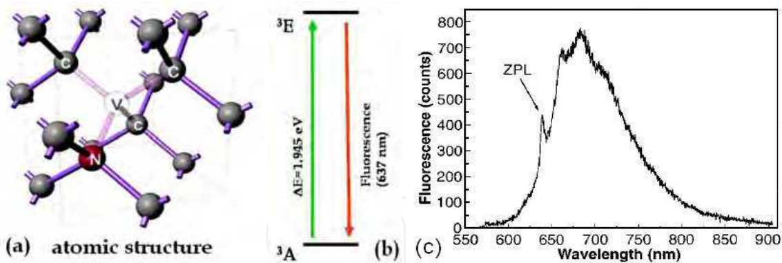
Fig. 1. a) Atomic structure of \text{NV}^- center in diamond (N=nitrogen V=Vacancy, C=Carbon) b) Energy level scheme of \text{NV}^- center. c) Fluorescence spectrum of a single \text{NV}^- defect center. The wavelength of the zero phonon line (ZPL) is 637\text{nm} ( 1.945\text{eV} ). Excitation was at 514\text{nm} (Image taken from Gruber et al. (1997))
