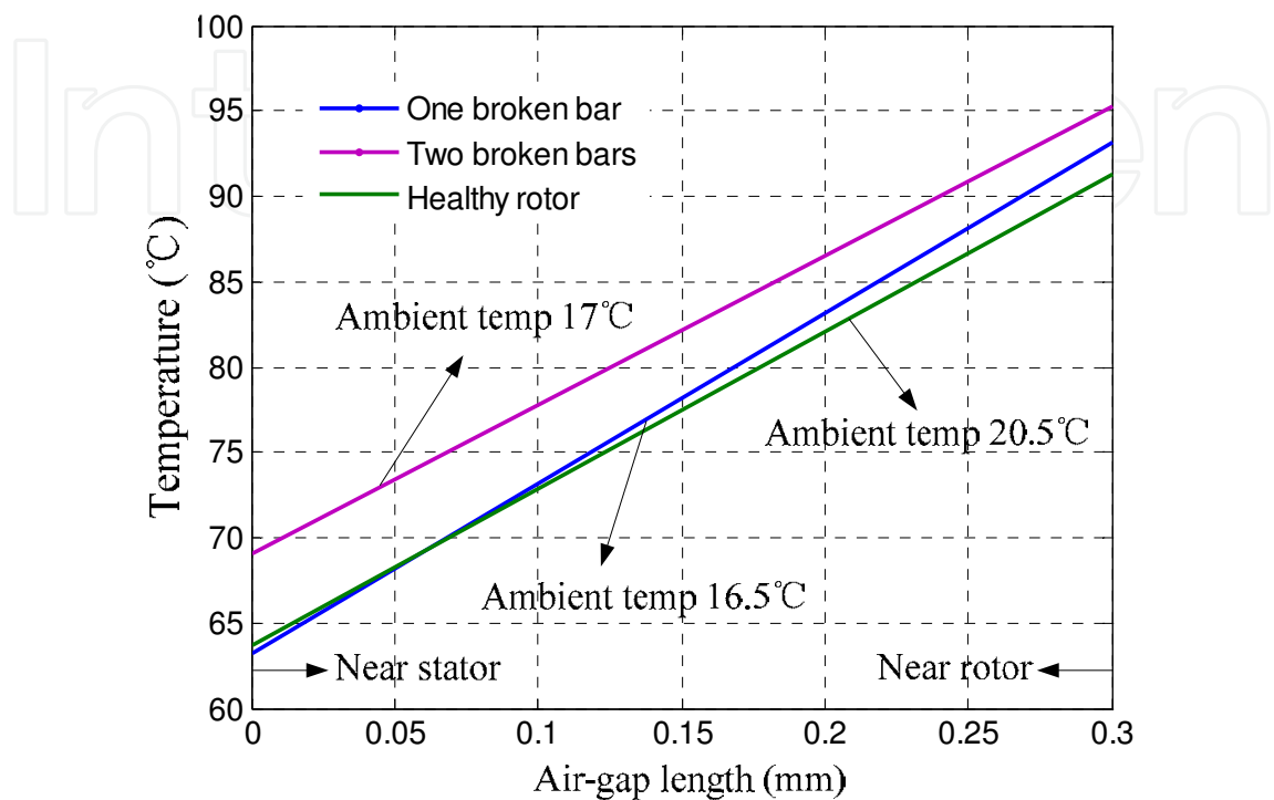
Fig. 25. The air-gap temperature distribution along radial
