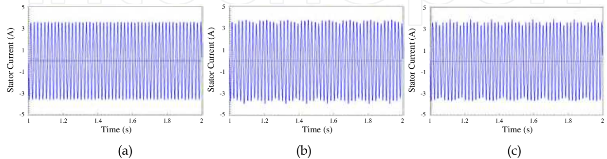
Fig. 10. The simulated stator current profile at rated load. (a) healthy rotor, (b) one broken bar, (c) two broken bars (ying xie 2009)
