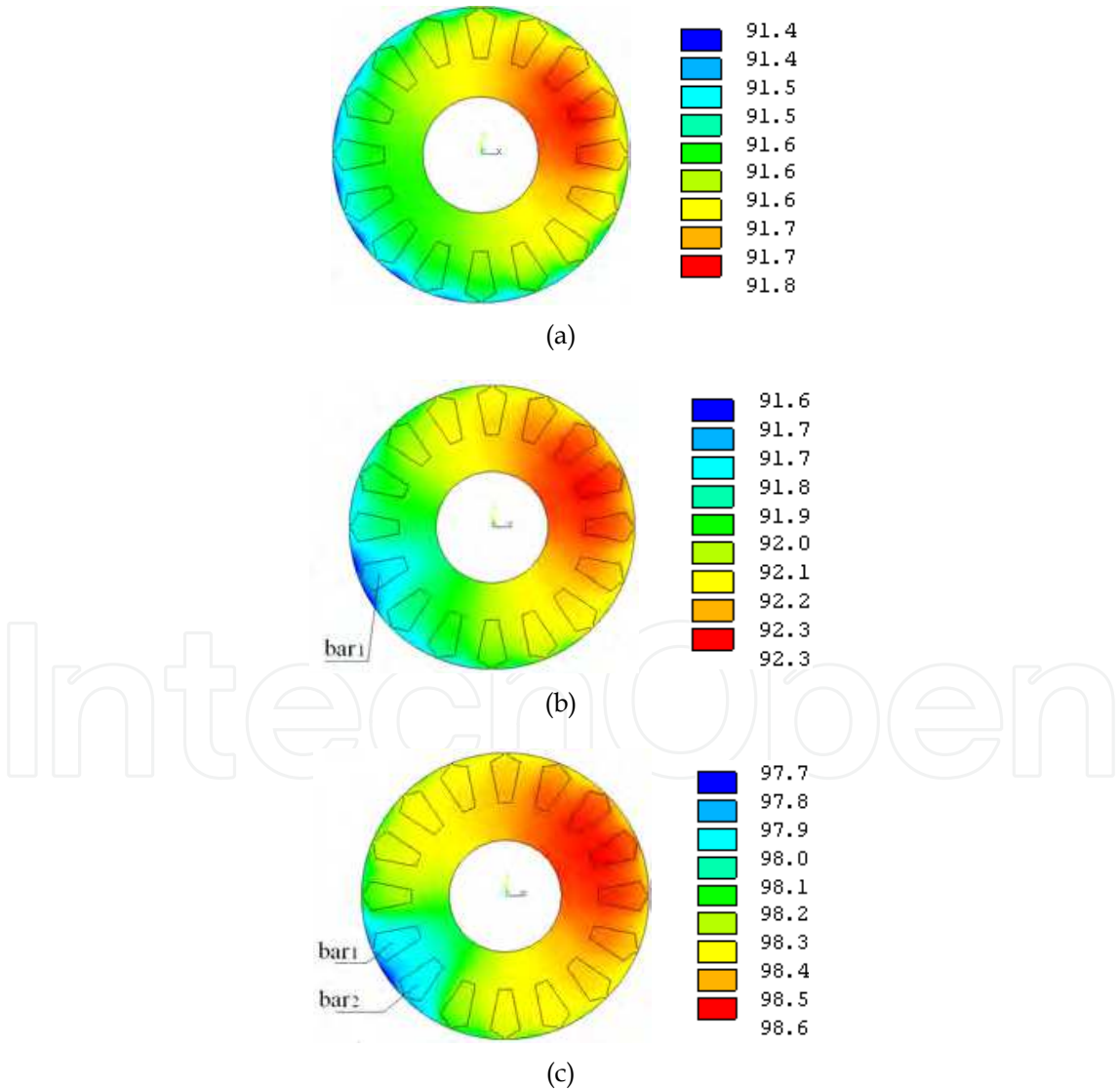
Fig. 24. Rotor temperature distribution. (a) healthy motor cage, (b) a bar 1 broken, (c) bar 1 and bar 2 broken (ying xie 2010)
