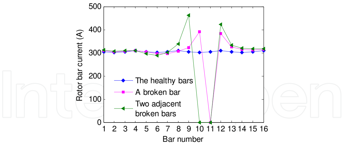
Fig. 13. The simulated rotor bar current at rated load.
