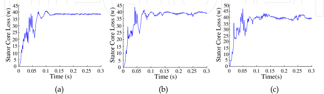
Fig. 20. Variations of stator core losses versus time before and after broken bars at rated load. (a) healthy motor cage, (b) a one-broken-bar fault, (c) a continuous two-broken-bar (ying xie, 2009)
