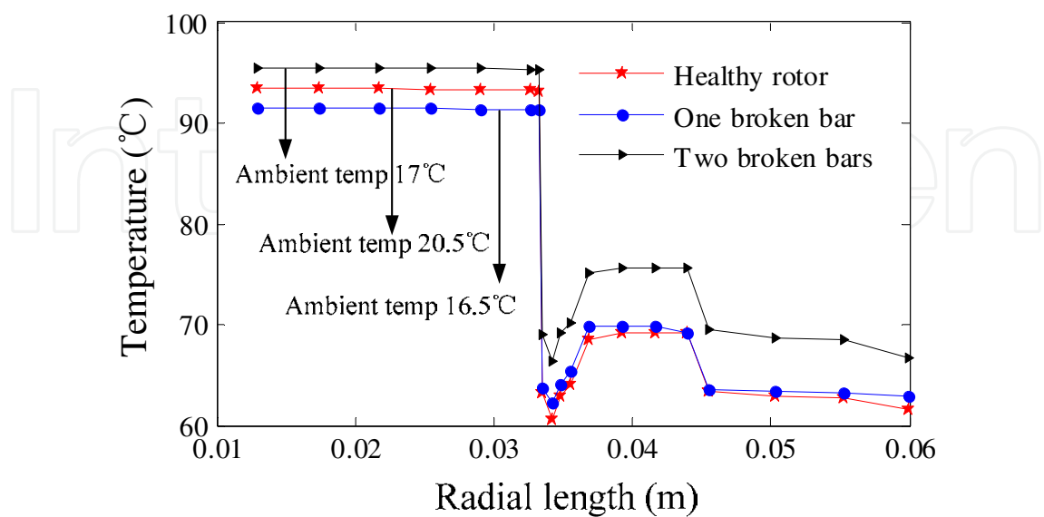
Fig. 26. Temperature distribution throughout radial
