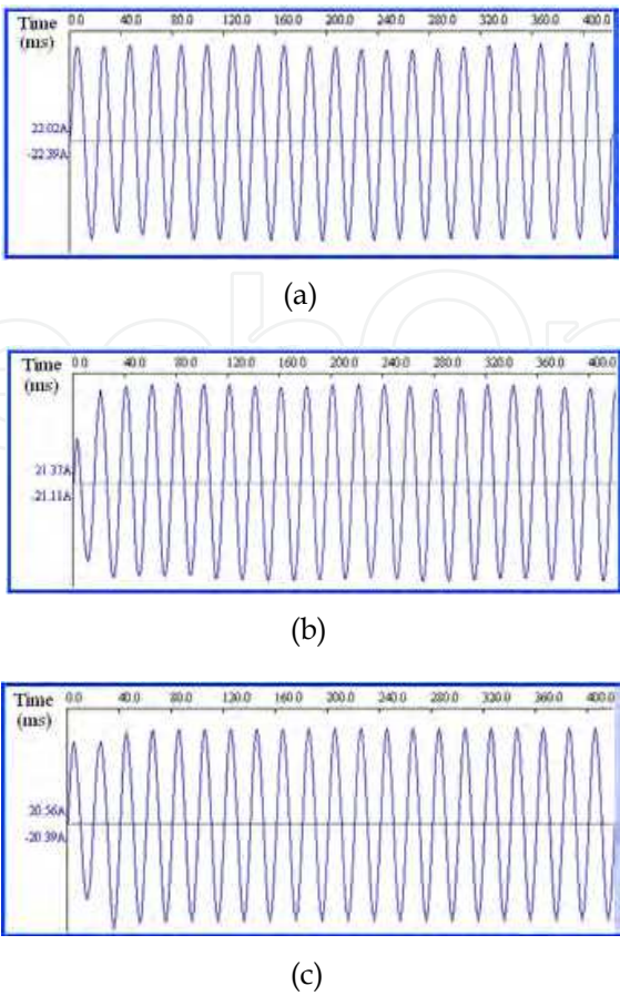
Fig. 11. The experimental stator current waveforms at standstill. (a) healthy rotor, (b) one broken bar, (c) two broken bars
