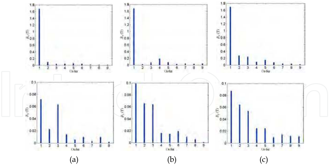
Fig. 7. The flux density frequency spectrum at position B at rated load. (a) healthy motor cage, (b) a one-broken bar fault, (c) a continuous two-broken-bar
