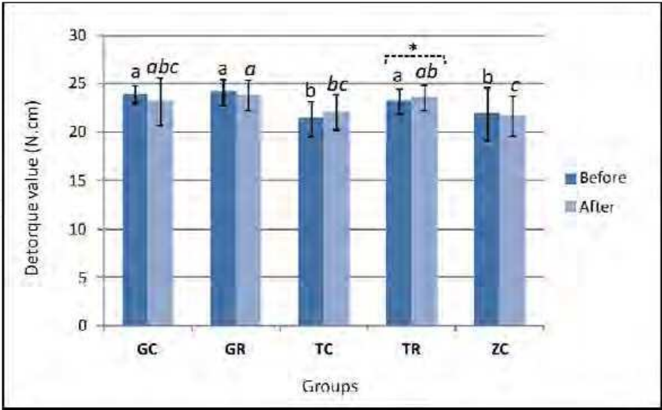
Fig. 4. Detorque mean value (N.cm) before and after mechanical cycling for all groups. Within each period, mean followed by different letters represent statistically significant difference ( P<.05 , Fisher’s exact test ).*denotes statistically significant difference within the same group ( P<.05 , Student's t-test ).
