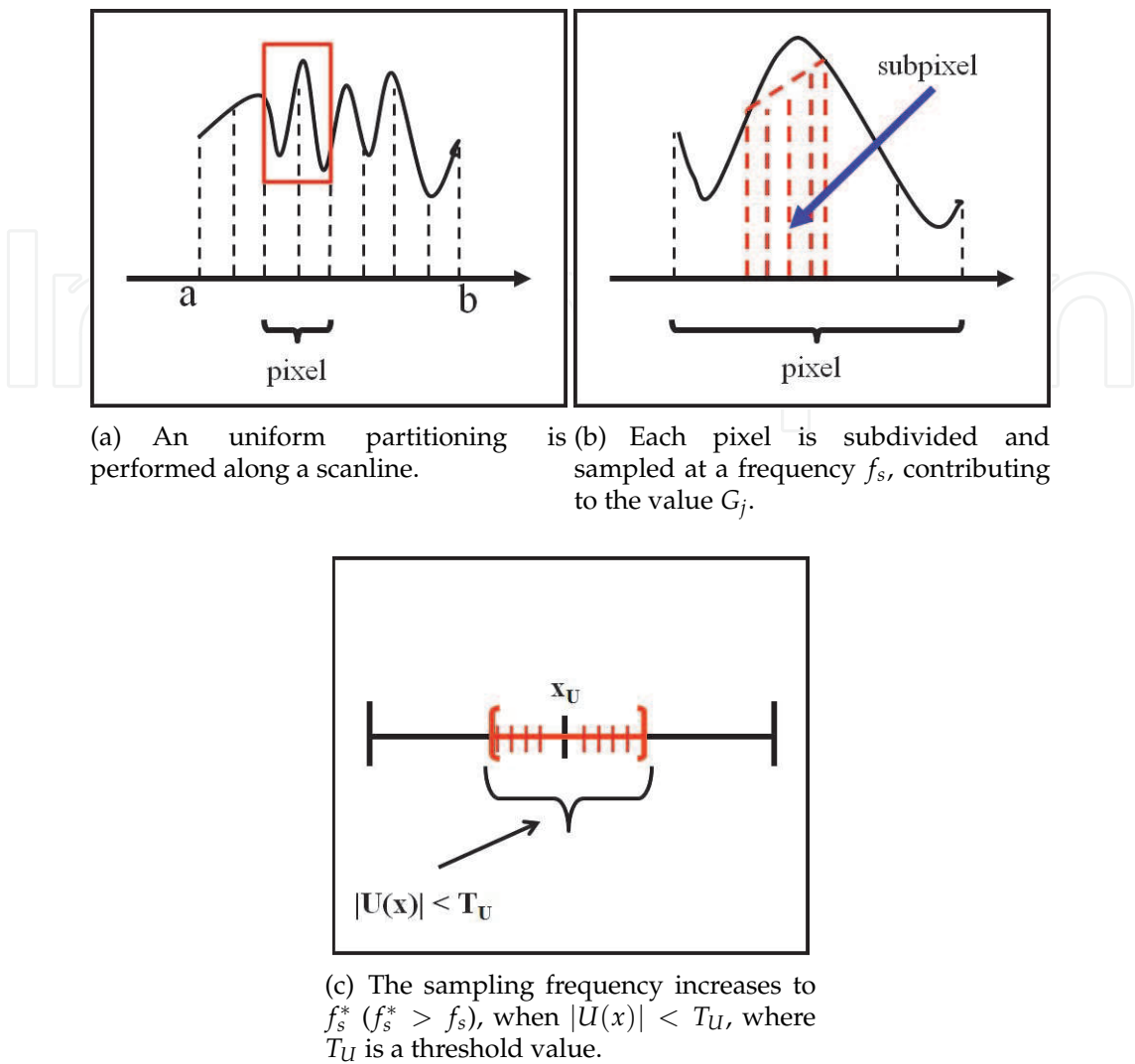
Fig. 6. Unweighted area sampling of the Green's function
