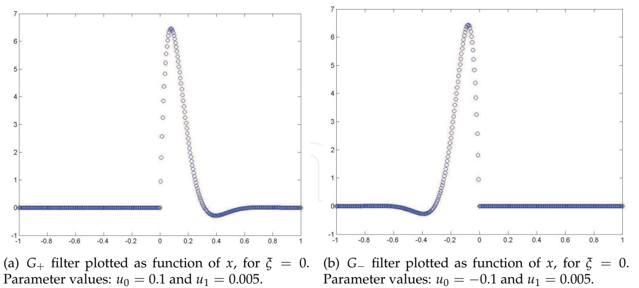
Fig. 3. Plots of the G_+ and G_- filters.
