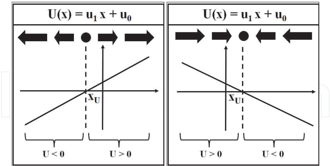
Fig. 1. Illustrating the behavior of the affine matching operator. Left: Expansion ( u_1 > 0 ). Right: Contraction ( u_1 < 0 ).
