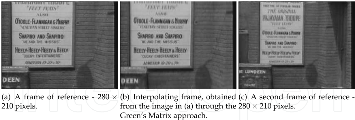
Fig. 9. Motion parameters were (u_0, u_1, v_0, v_2) = (-0.015, 0.000, -3, 0.029) . A focus of expansion appears at (x_U, y_V) = (140, 105) .
