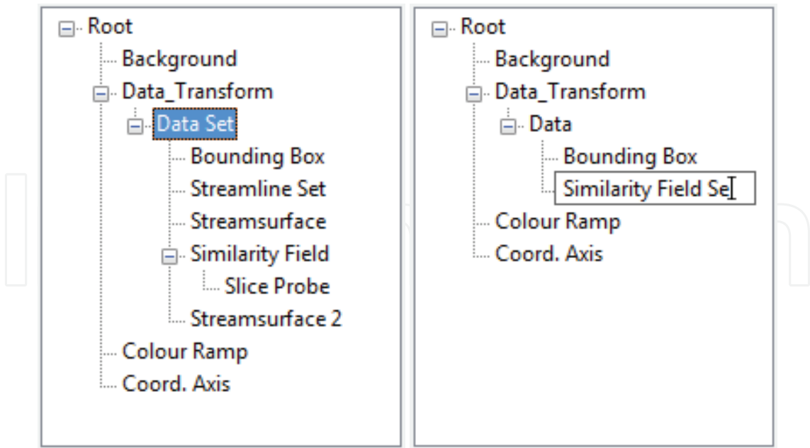
Fig. 8. Screenshots of the application tree during the run-time of different sessions. The application tree is a GUI tree control that represents the nodes in the scene graph. (Left) Several visualization assets, such as streamline sets and slice probes, are currently being employed. (Right) The user is editing the label of one of the assets.
