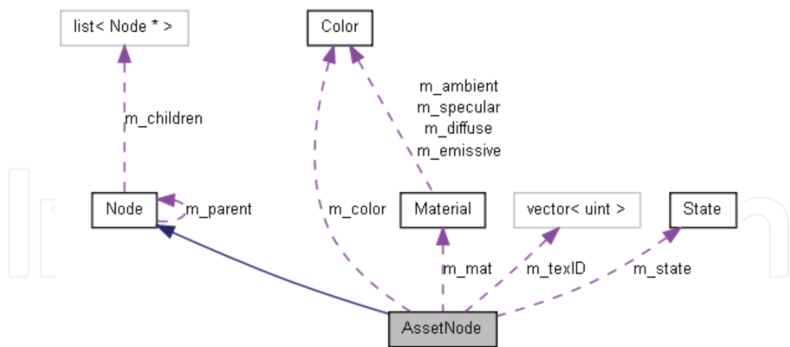
Fig. 10. Collaboration diagram for the asset node class. The boxes represent classes in our framework.
