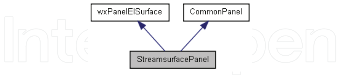
Fig. 12. Inheritance diagram for asset panel types. This example shows the streamsurface panel. Asset panels use multiple inheritance, they inherit from CommonPanel and another class that is auto-generated using a GUI builder. Using this method provides fast creation of GUI controls (using the form builder and generated class) and allows us to provide a common interface and behavior for all panels (using the common panel class). panel then provides the implementation for the interface. In our system the auto-generated classes are prefixed with the letters "wx" to differentiate them from user created classes.
