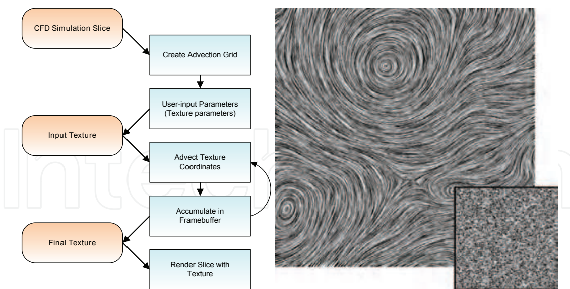
Fig. 5. (Left) The processing pipeline for the texture-based visualization subsystem. (Right) A Line Integral Convolution (LIC) visualization using the texture-based visualization system. This image was generated by ‘smearing’ the noise texture (inset) along the direction of the underlying vector field at each pixel. The visualization is of a simulation of Hurricane Isabel. The eye of the hurricane can be seen towards the top of the image.
