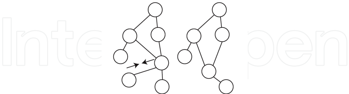
Fig. 10. Edge collapsed and merged into one single node.
