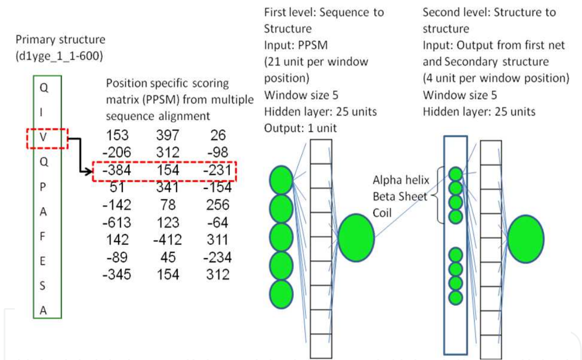
Fig. 3. An example of secondary structure prediction using BRNN.
