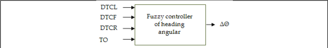
Fig. 4. Fuzzy controller of heading angular
