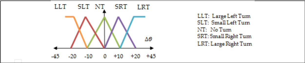
Fig. 6. The definition of angular velocity output membership functions.
