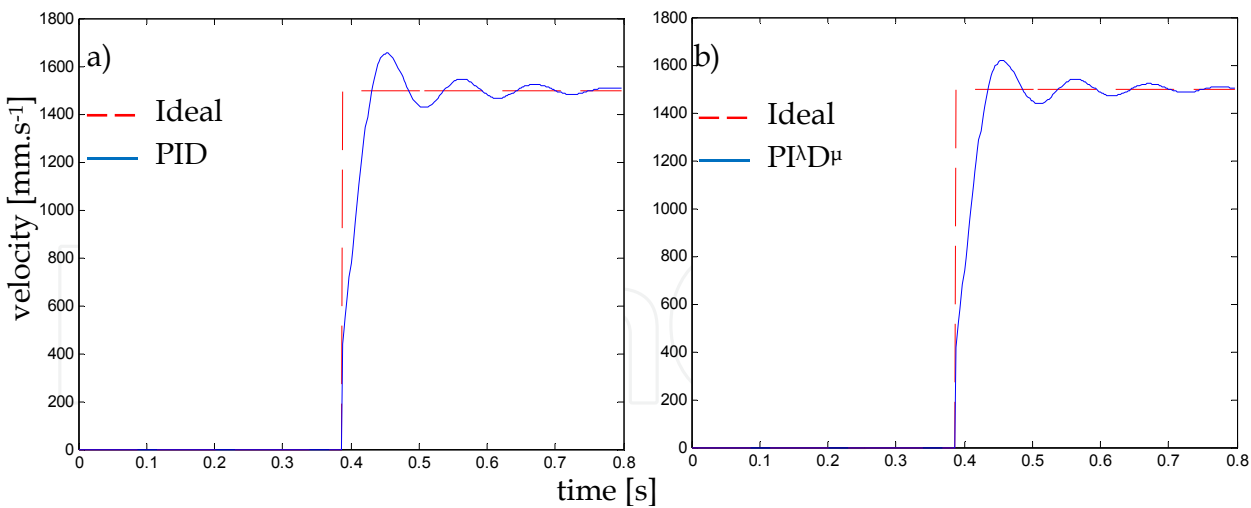
Fig. 7. Time response of the device with a putting impact velocity of 1500 mm.s -1 under the action of the: a) PID controller; b) PI λ D μ controller.
