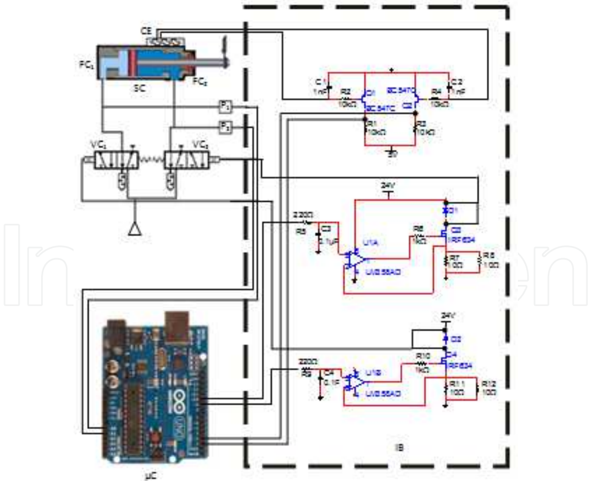
Fig. 3. Schematic of the Putting Mechanism.
