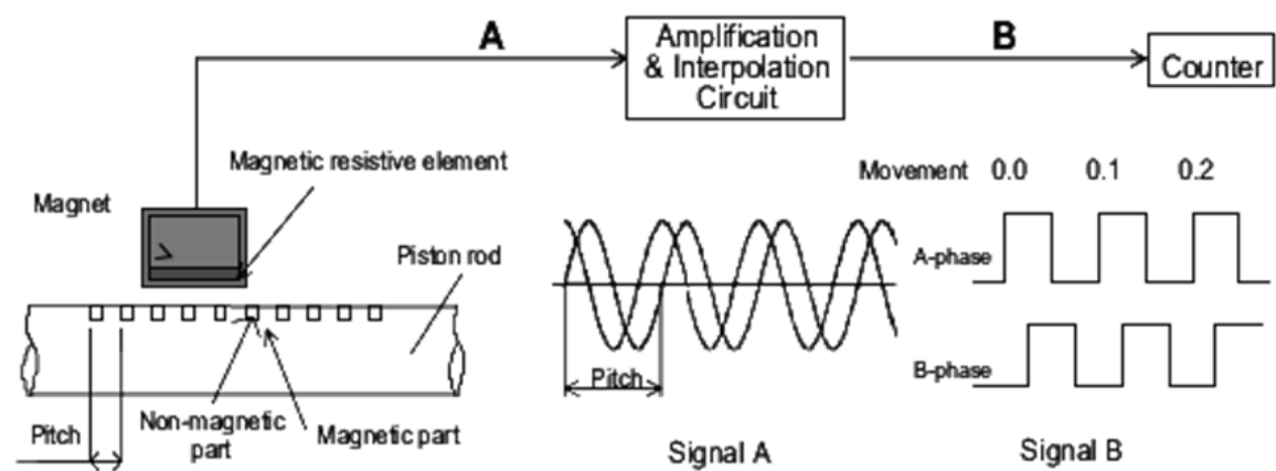
Fig. 4. Feedback System using encoders.
