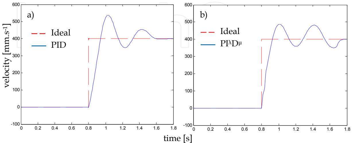
Fig. 6. Time response of the device with a putting impact velocity of 400 mm.s -1 under the action of the: a) PID controller; b) PI λ D μ controller.
