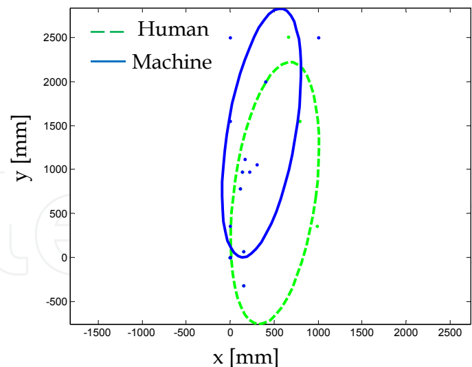
Fig. 9. Error Ellipse of 30 trials performed by an expert golf player and subsequently emulated by the putting mechanism.
