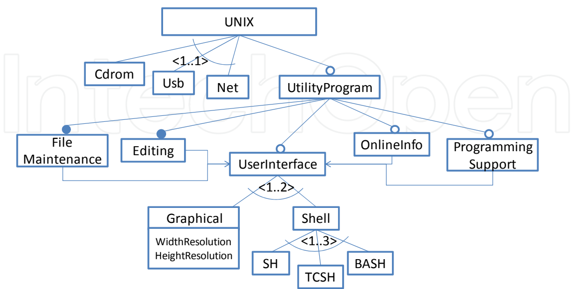
Fig. 1. User model of the UNIX operating system family of our running example
