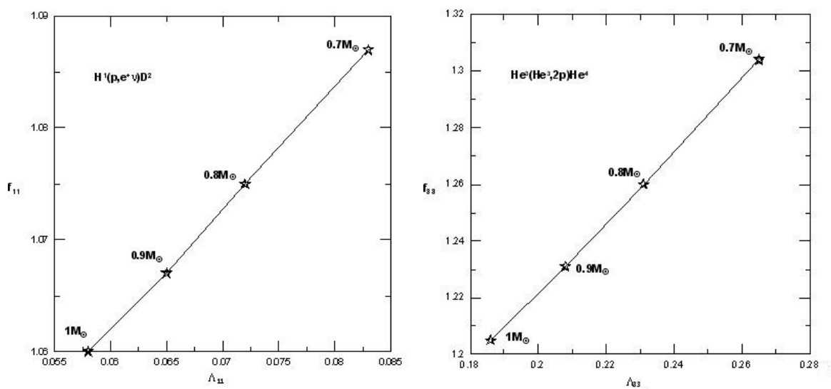
Fig. 1. Variation of the screening factors (S54) for H^1(p,e^+\nu)D^2 reaction with the screening strength parameter \Lambda (left). Variation of the screening factors (S54) for He^3(He^3,2p)He^4 reaction with the screening strength parameter (right)
