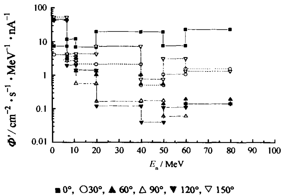
Fig. 18. Measured neutron spectra of 78MeV/u 12 C on thick Au target with threshold detectors The development of scintillation detector and nanosecond pulse technology makes it possible to measure high energy neutron with time-of-flight (TOF) method. T.Kurosawa et.al reported the neutron spectra experiment of 800MeV/u Ne bombarded with thick target [12]. In particle therapy, maximum neutron energy will approach about 1GeV. TOF method is the best way to obtain neutron spectrabut it needs enough flight space to get good energy solution.
