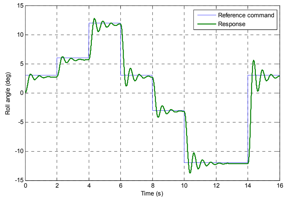
Fig. 6. PID controller performance at normal speed (12km/h)
