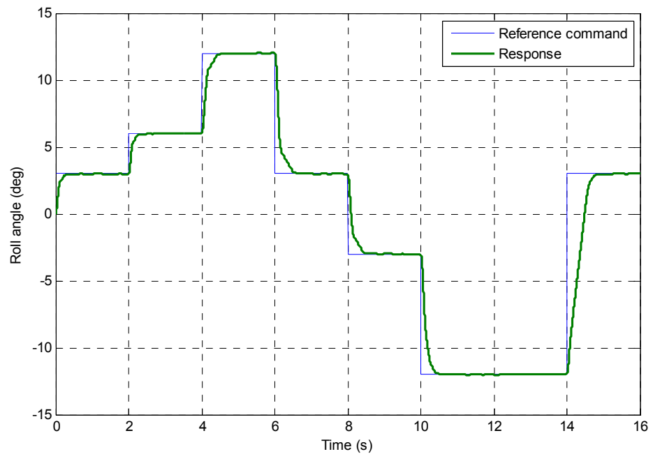
Fig. 7. Roll-angle-tracking performance at low speed (5km/h)
