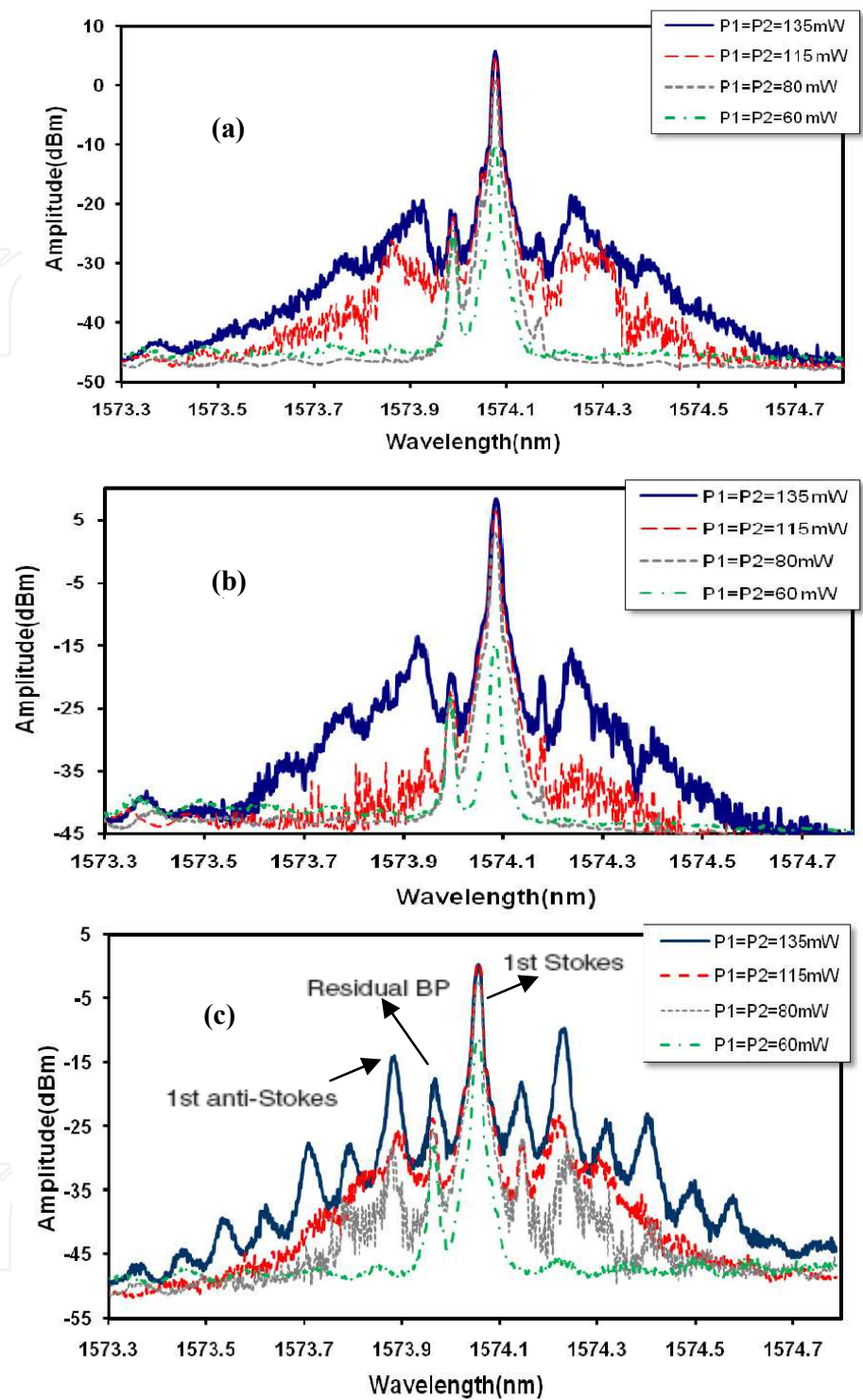
Fig. 5. The BFL output spectrum for (a) 80/20 coupler, (b) 90/10 coupler and (c) 95/5 coupler. Both pumps are at the same power for each output coupling ratio. frequency. The representation of this image can be observed in Figures 5 where the multi-wavelength spectrum is more symmetry with the use of 95/5 output coupler.
