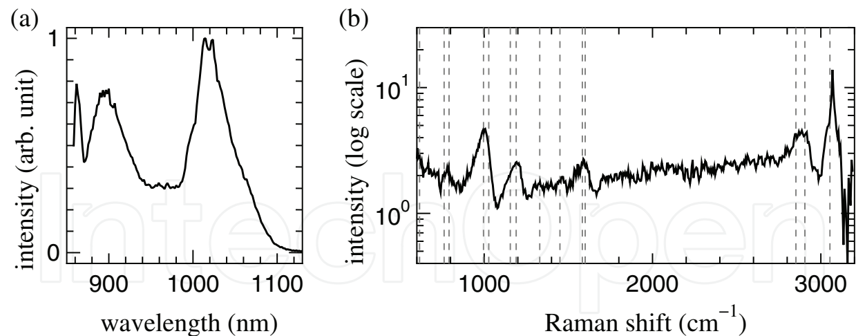
Fig. 12. (a) The spectrum of quasi-SC. (b) The normalized CARS spectrum using quasi-SC of a 6-μm diameter polystyrene bead sample. Peak positions of spontaneous Raman spectrum are shown by dashed lines.
