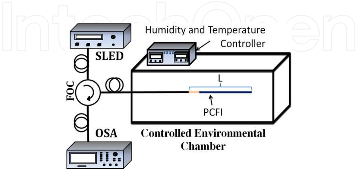
Fig. 5. Experimental arrangement for the characterisation of the PCFI with respect to relative humidity.
