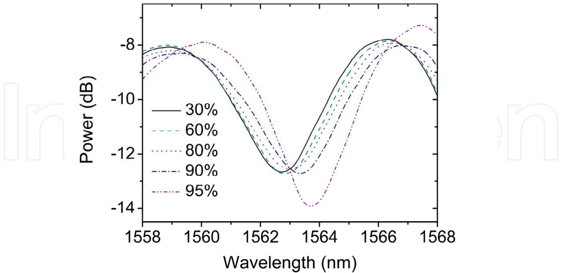
Fig. 6. Reflection spectrum of a 40.5 mm long PCFI at different humidity values.
