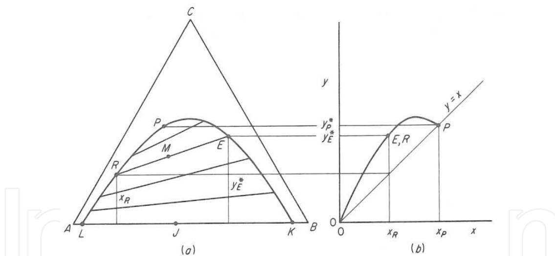
Fig. 17. Triangular (a) and distribution diagram (b) for liquid-liquid equilibria for a system of three components where one pair is partially miscible (extracted from Treybal, 1981).
