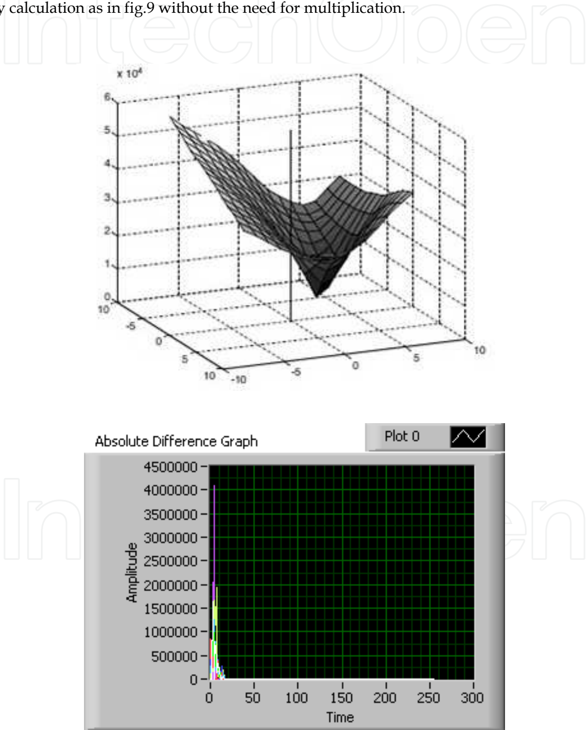
Fig. 9. SAD Map & its PSNR sketch
