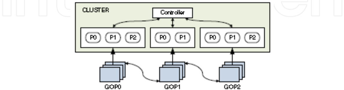
Fig. 12. Frame-level Parallelism
