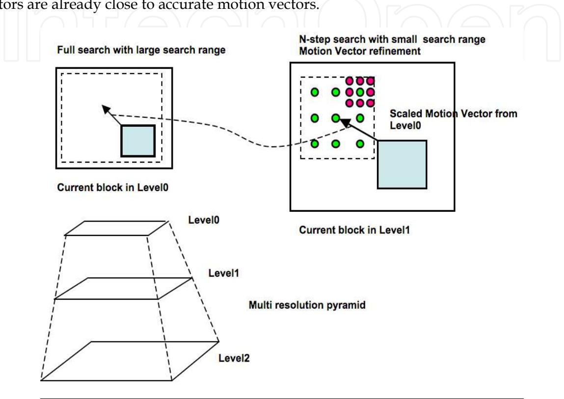
Fig. 4. Hierarchical block matching
