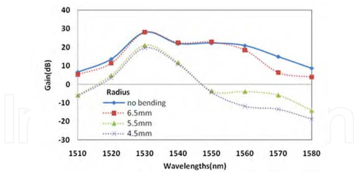
Fig. 6. Efficient length of EDF (3m) in different bending radius for -30dBm input signal]
