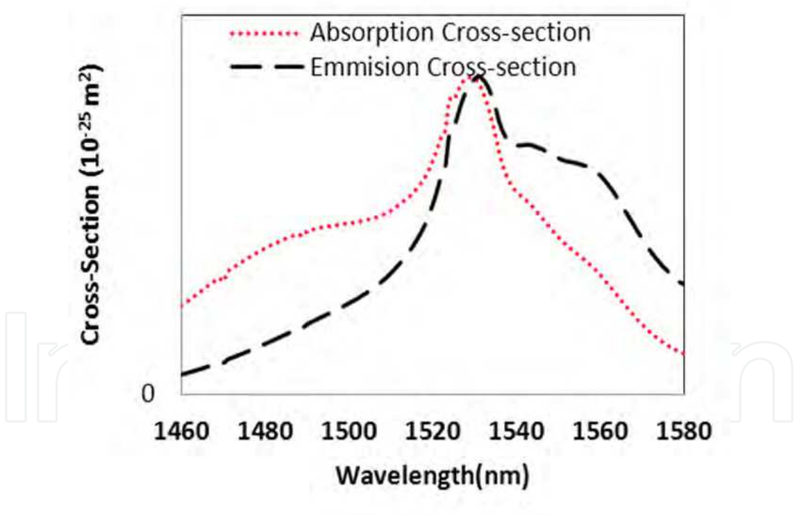
Fig. 12. Absorption and Emission Cross section.
