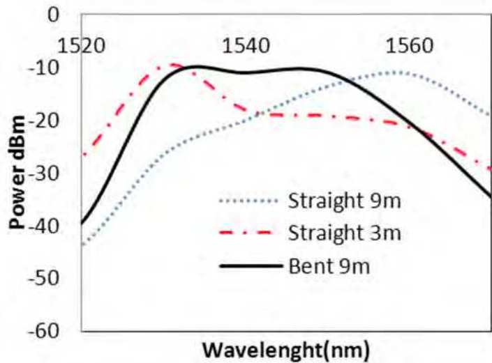
Fig. 18. Amplified Spontaneous emission (Simulation)
