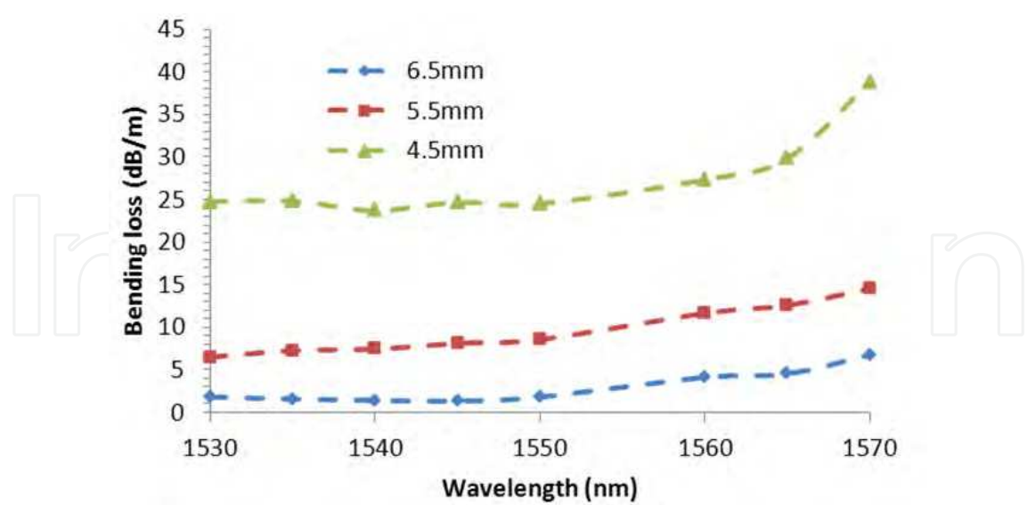
Fig. 5. Bending loss (dB/m) vs. wavelength (nm) for different bending radius
