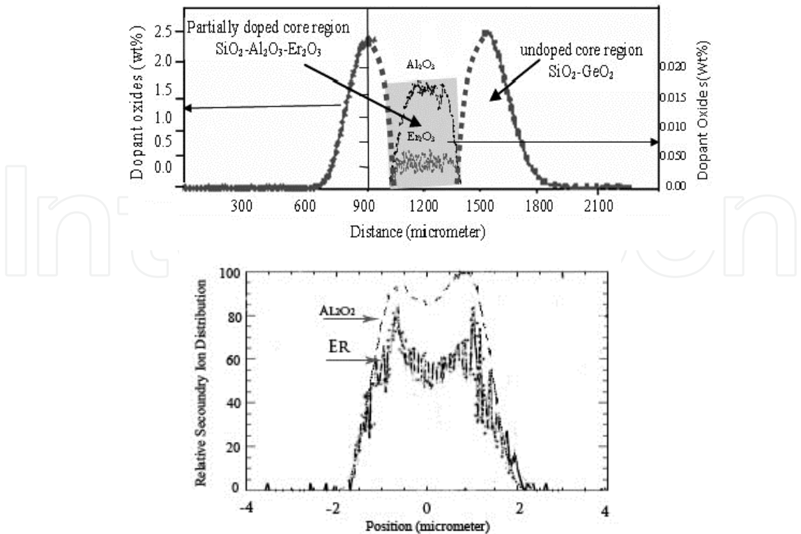
Fig. 25. Erbium TDP. (a) 2µm doping radius (b) 4µm doping
