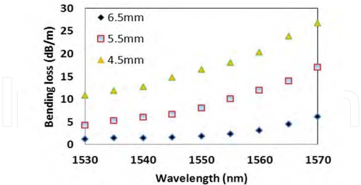
Fig. 13. Bending loss spectral for different bending radius
