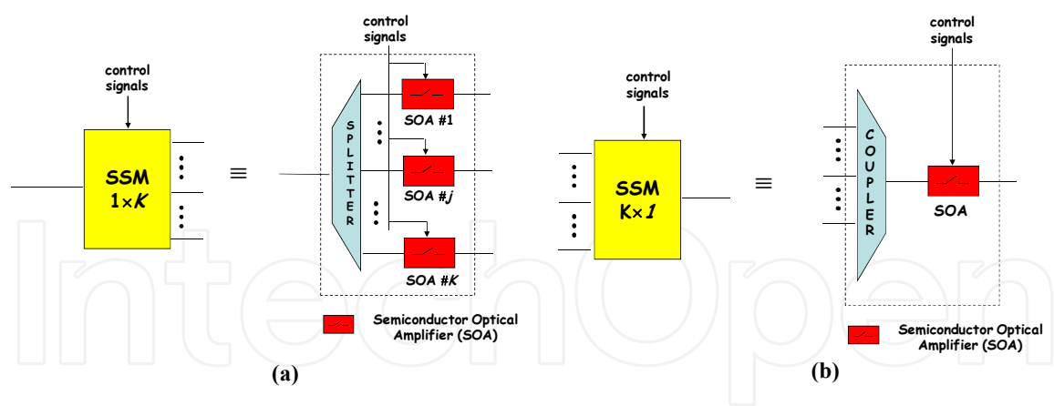
Fig. 7. Realization of 1 \times K SSM (a) and K \times 1 SSM (b) by means of splitters, couplers and Semiconductor Optical Amplifiers (SOA).
