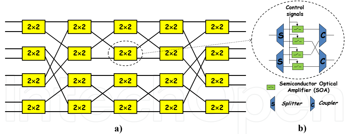
Fig. 8. 8 \times 8 BENES switching architecture realized with 20 2 \times 2 switching elements (a). SOA technology based 2 \times 2 switching element (b).
