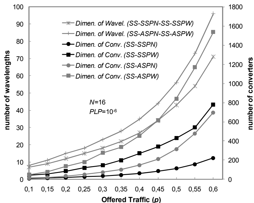
Fig. 11. Dimensioning of wavelengths and WCs in SS-ASPW, SS-ASP-SSPN, SS-SSPW and SS-SSPN switches so that the PLP is smaller than or equal to 10^{-6} . The number N of Input/Output Fibers equal 16 and the offered traffic \rho is varying from 0,1 to 0,6.
