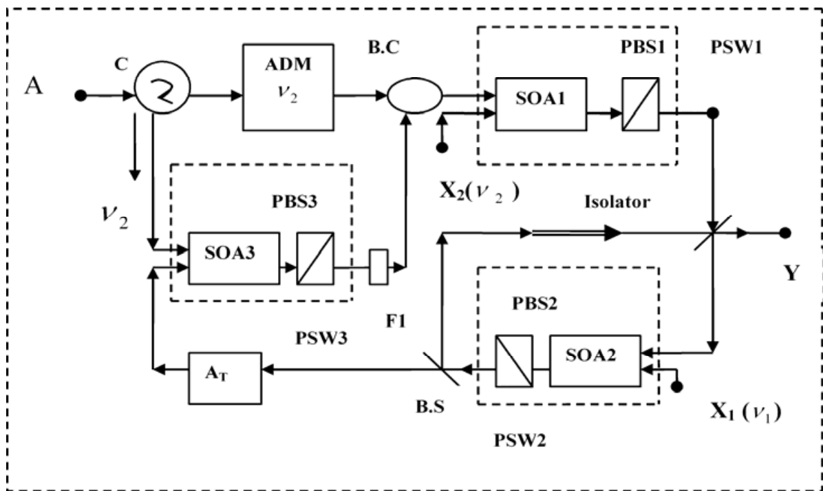
Fig. 5. Frequency encoded single bit memory circuit
