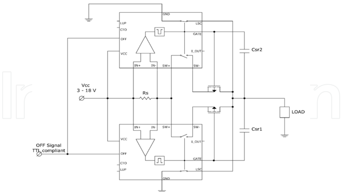
Fig. 11. Advanced protection stage with redundancy of protection modules and external transistors. A simple system can use just one device plus an external resistor.
