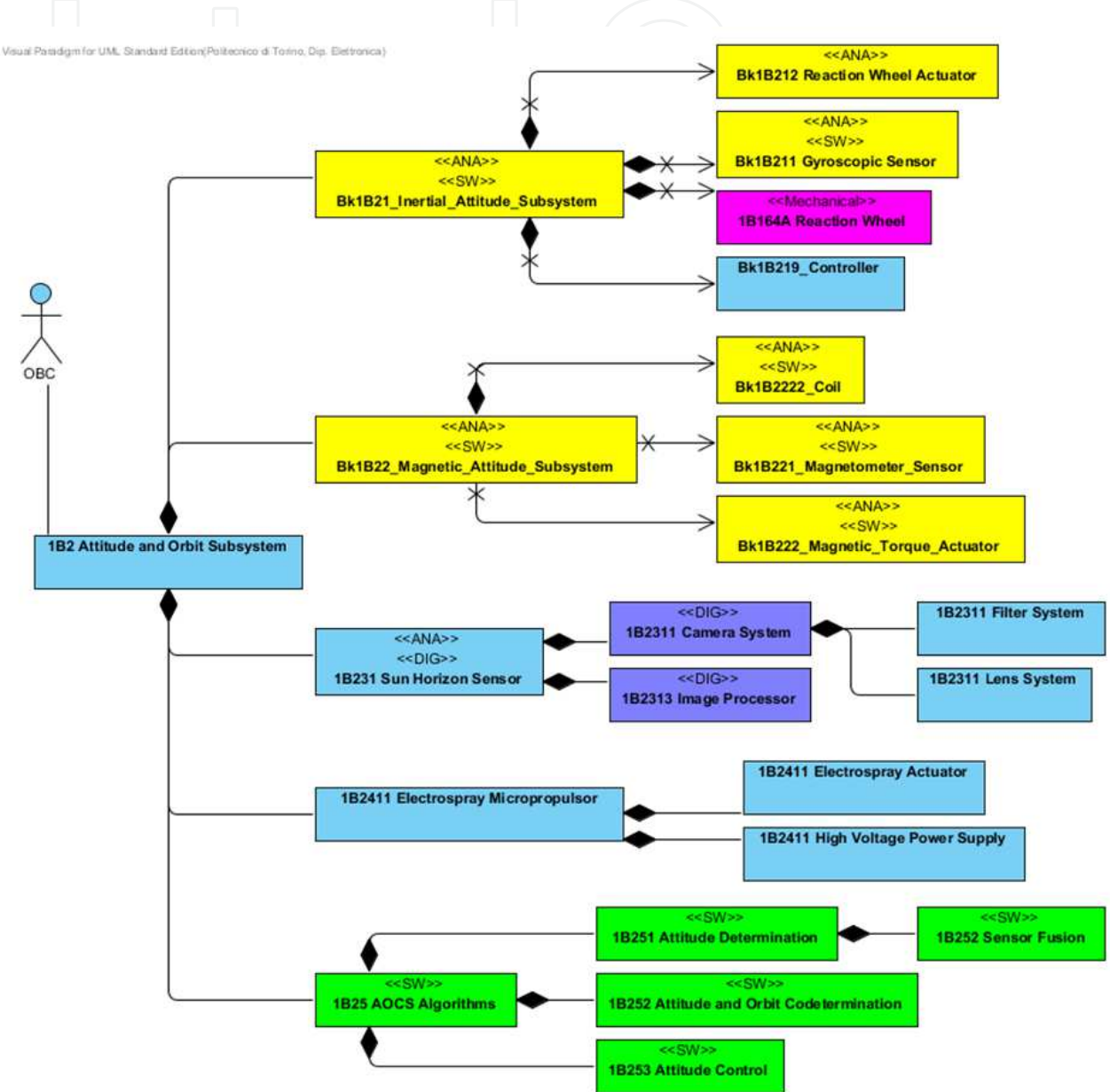
Fig. 2. Overview of the proposed Attitude and Orbit Control System.
