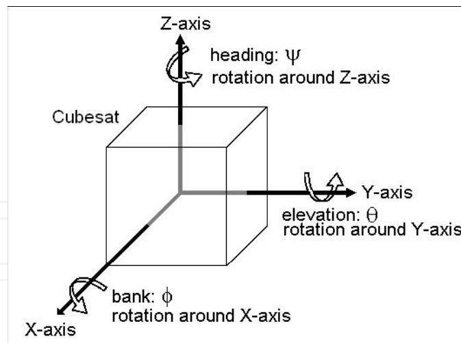
Fig. 3. Satellite coordinate system and Euler angles.
