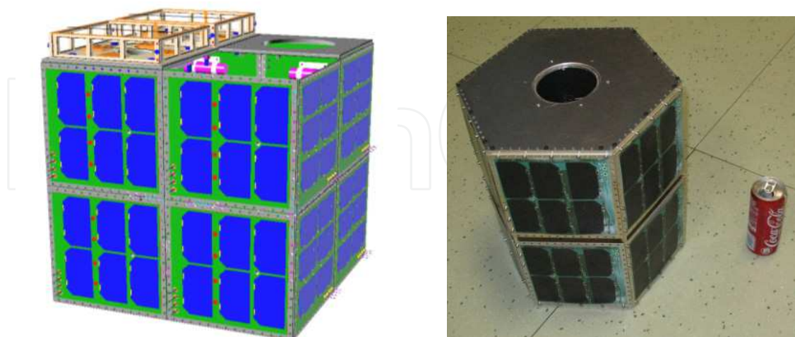
Fig. 1. Mechanical sketch of a 2x2x2 cubic configuration using 22 tiles (left). Photograph of the mockup of a hexagonal telescope made using 12 tiles.
