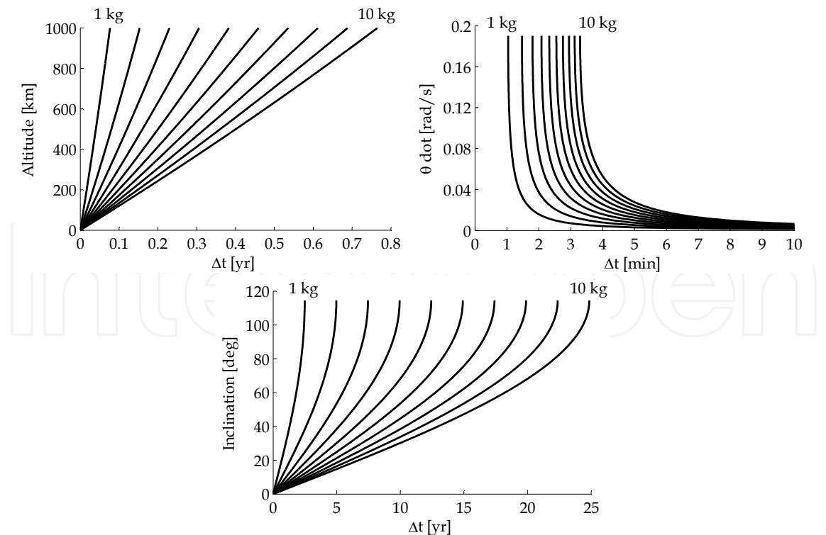
Fig. 14. Maneuver time of chosen micropropulsor for three different attitude and orbit maneuvers: deorbiting (left); spin (right); orbital plane inclination (bottom). All plots are for satellite masses from 1 kg to 10 kg.
