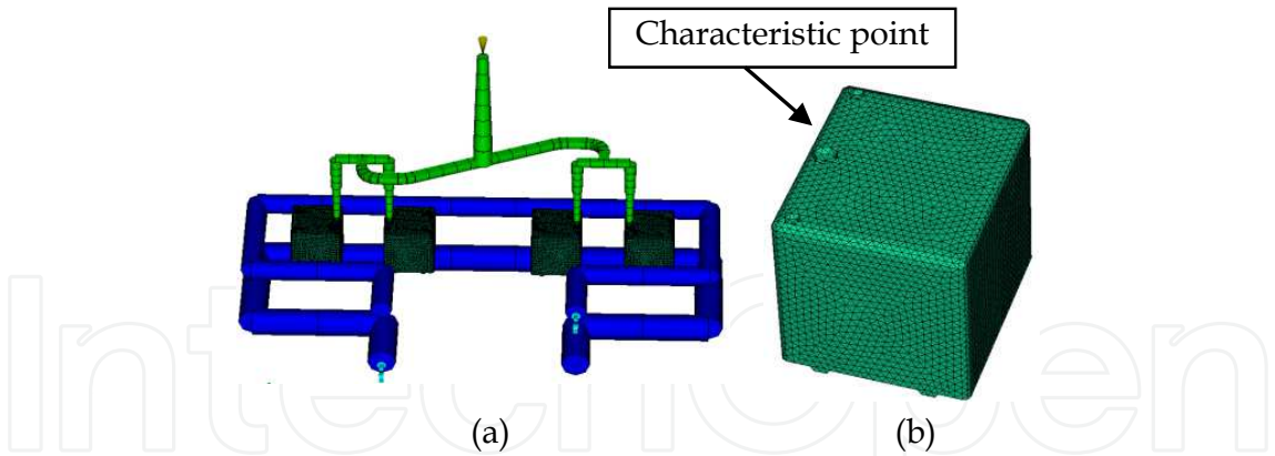
Fig. 2-2. Experimental model and characteristic point position (a): CAE analysis model; (b): Characteristic point position.
