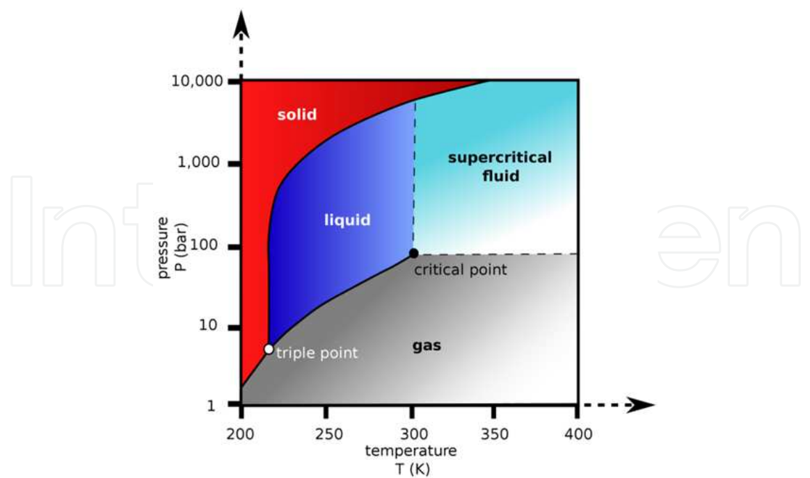
Fig. 2-1. Carbon dioxide pressure-temperature phase diagram [30].
