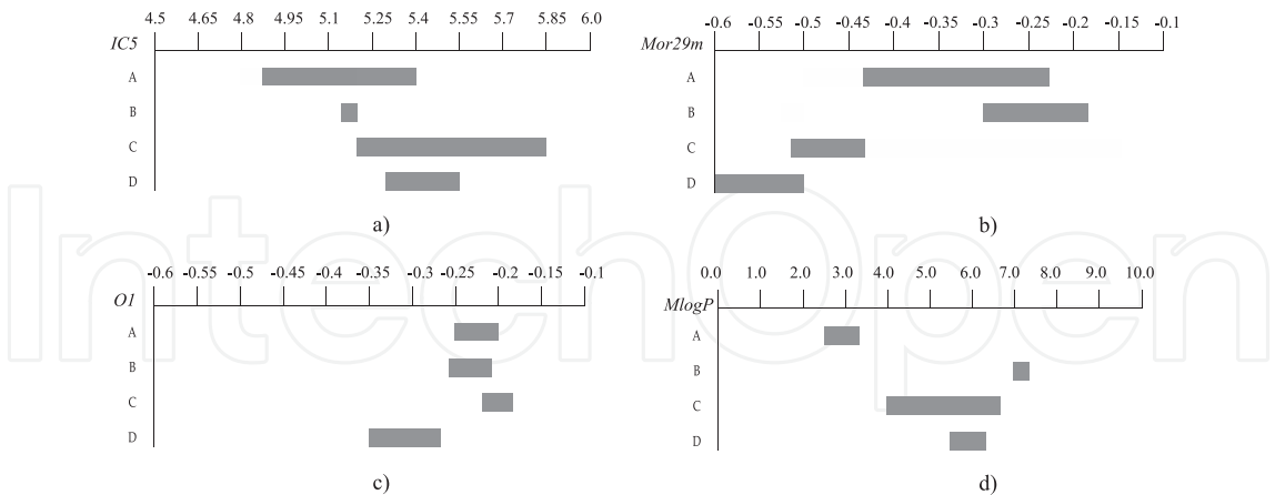
Fig. 9. Variations in descriptors: a) Variations in IC5 for each cluster; b) Variations in Mor29m for each cluster; c) Variations in OI for each cluster; d) Variations in MlogP for each cluster
