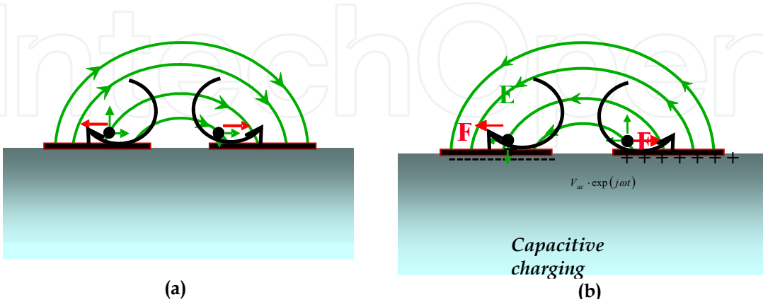
Fig. 2. ACEO fluid motion and induced charge at electrode surface. (a) during the half cycle when the left electrode has positive polarity; (b) during the next half cycle with opposite electrical polarity.
